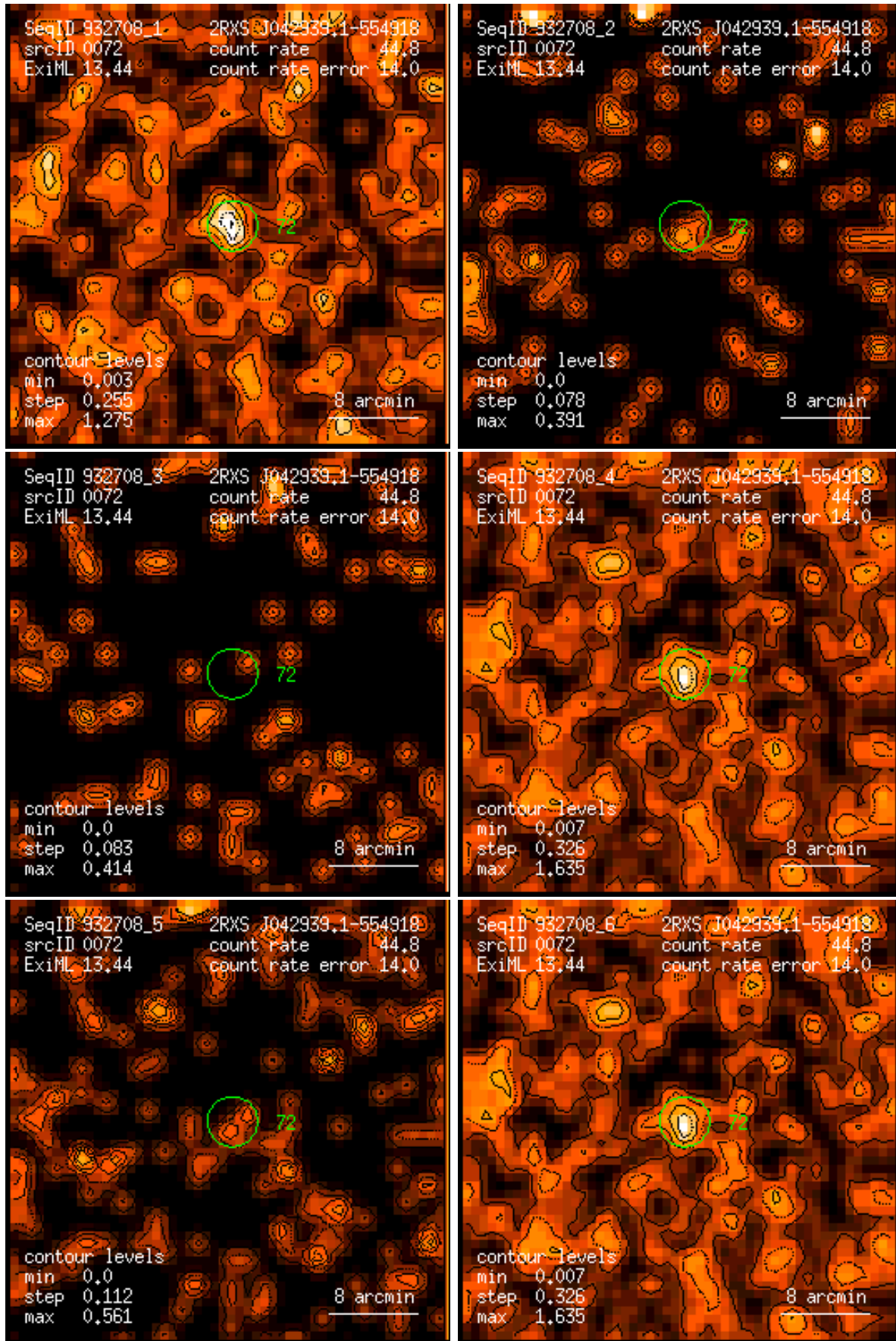
Figure 72: RASS 932708: detection 0072: band rate images, Gaussian filter: (1) PSPC channels 11 – 41, (2) 52 – 90, (3) 91 – 201, (4) 11 – 235, (5) 52 – 201, (6) 11 – 201. Broad band rates in counts/ks. Band rate contour levels in counts/ks/arcmin 2 .
