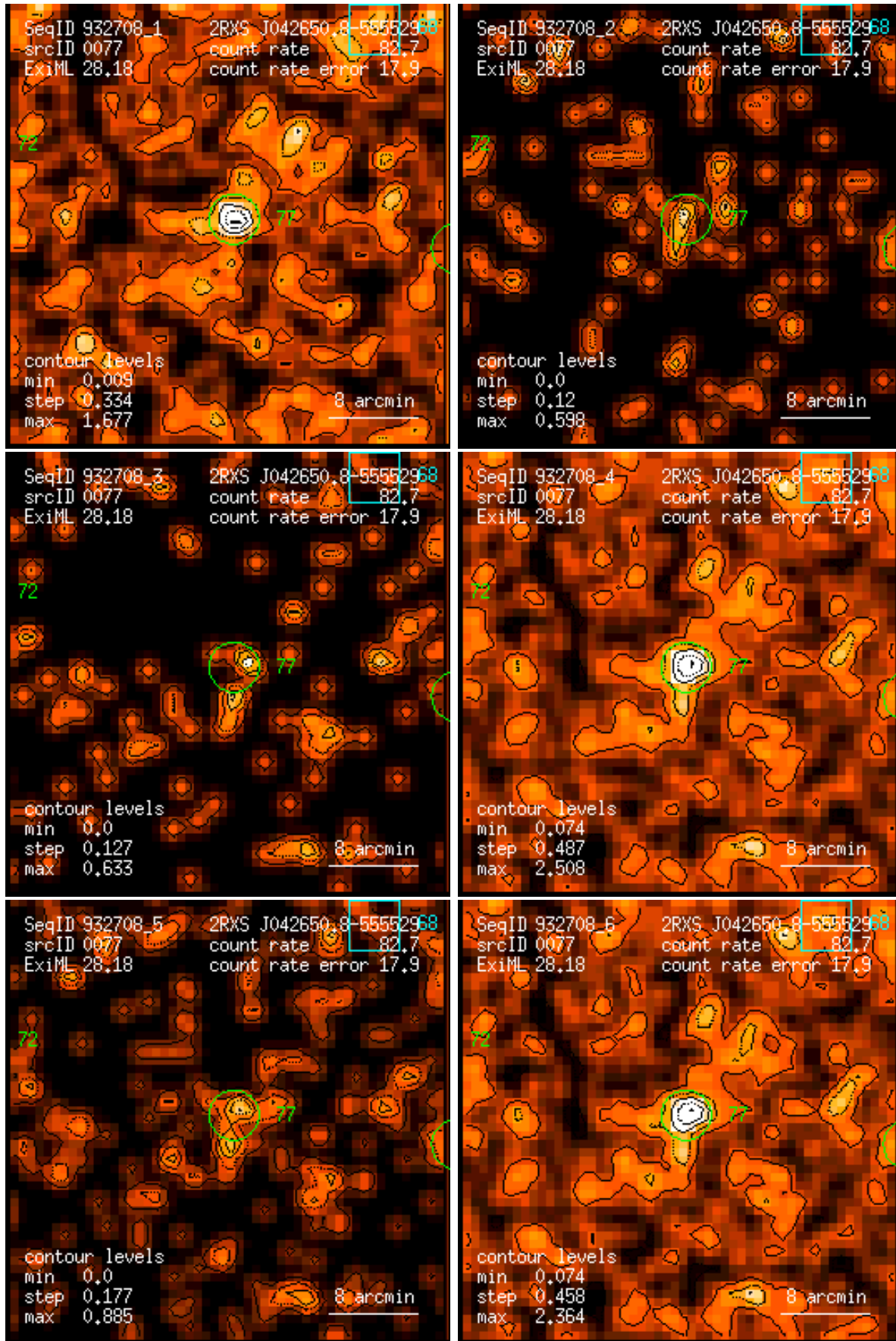
Figure 77: RASS 932708: detection 0077: band rate images, Gaussian filter: (1) PSPC channels 11 – 41, (2) 52 – 90, (3) 91 – 201, (4) 11 – 235, (5) 52 – 201, (6) 11 – 201. Broad band rates in counts/ks. Band rate contour levels in counts/ks/arcmin 2 .
