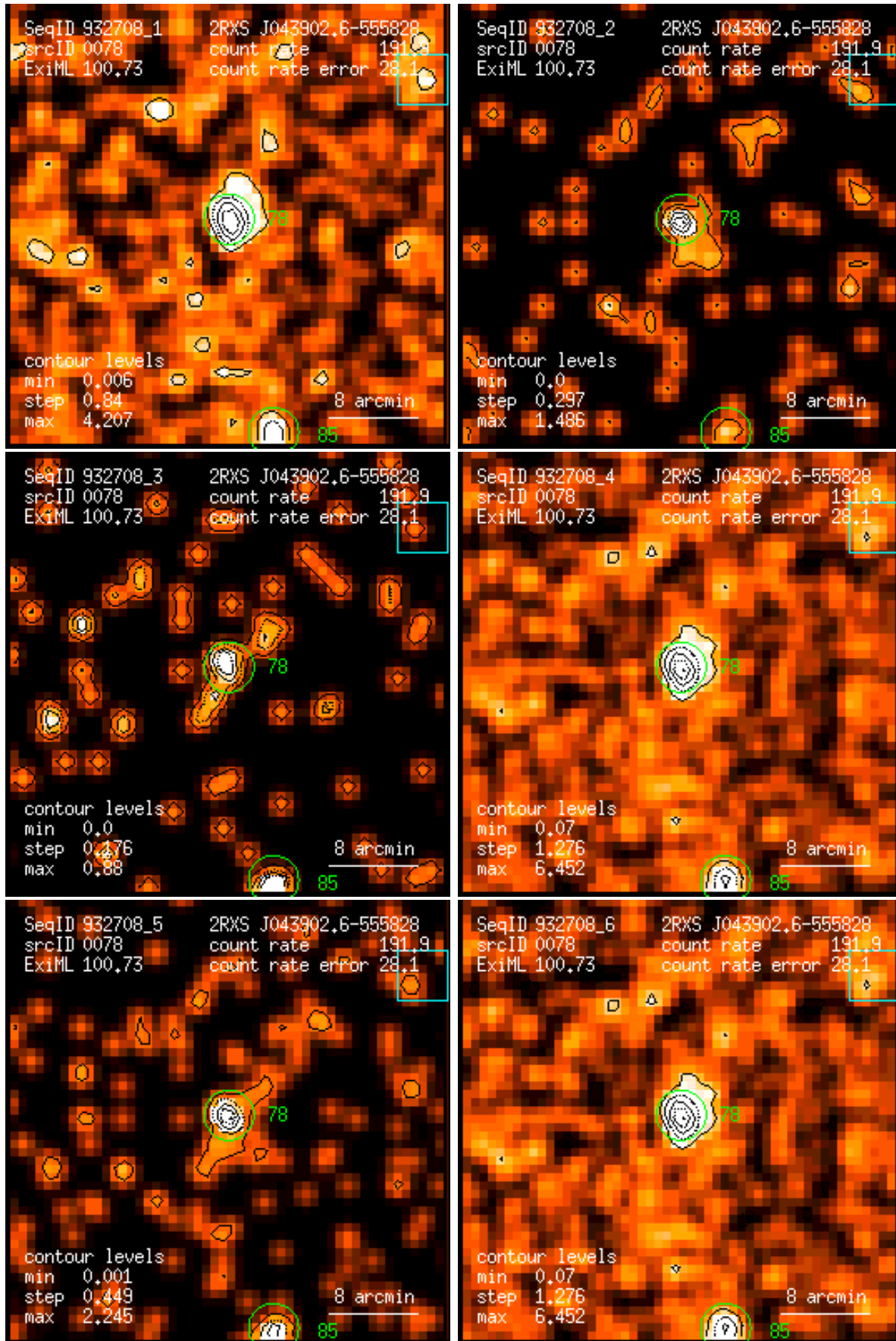
Figure 78: RASS 932708: detection 0078: band rate images, Gaussian filter: (1) PSPC channels 11 – 41, (2) 52 – 90, (3) 91 – 201, (4) 11 – 235, (5) 52 – 201, (6) 11 – 201. Broad band rates in counts/ks. Band rate contour levels in counts/ks/arcmin 2 .
