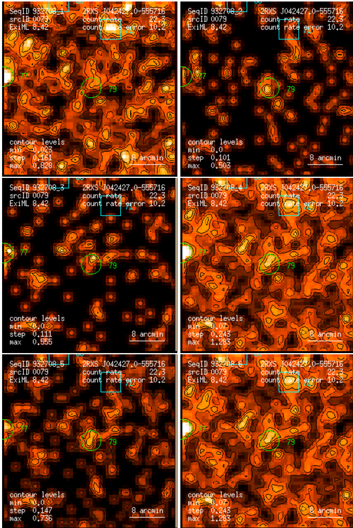
Figure 79: RASS 932708: detection 0079: band rate images, Gaussian filter: (1) PSPC channels 11 – 41, (2) 52 – 90, (3) 91 – 201, (4) 11 – 235, (5) 52 – 201, (6) 11 – 201. Broad band rates in counts/ks. Band rate contour levels in counts/ks/arcmin 2 .
