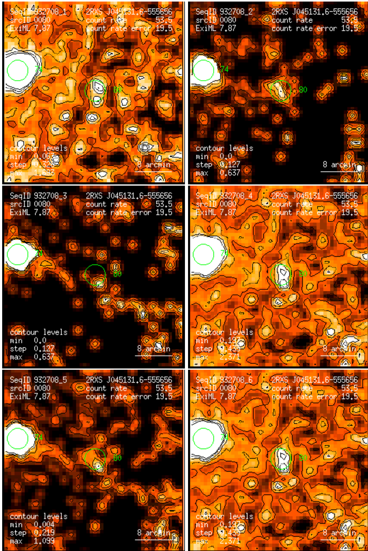
Figure 80: RASS 932708: detection 0080: band rate images, Gaussian filter: (1) PSPC channels 11 – 41, (2) 52 – 90, (3) 91 – 201, (4) 11 – 235, (5) 52 – 201, (6) 11 – 201. Broad band rates in counts/ks. Band rate contour levels in counts/ks/arcmin 2 .
