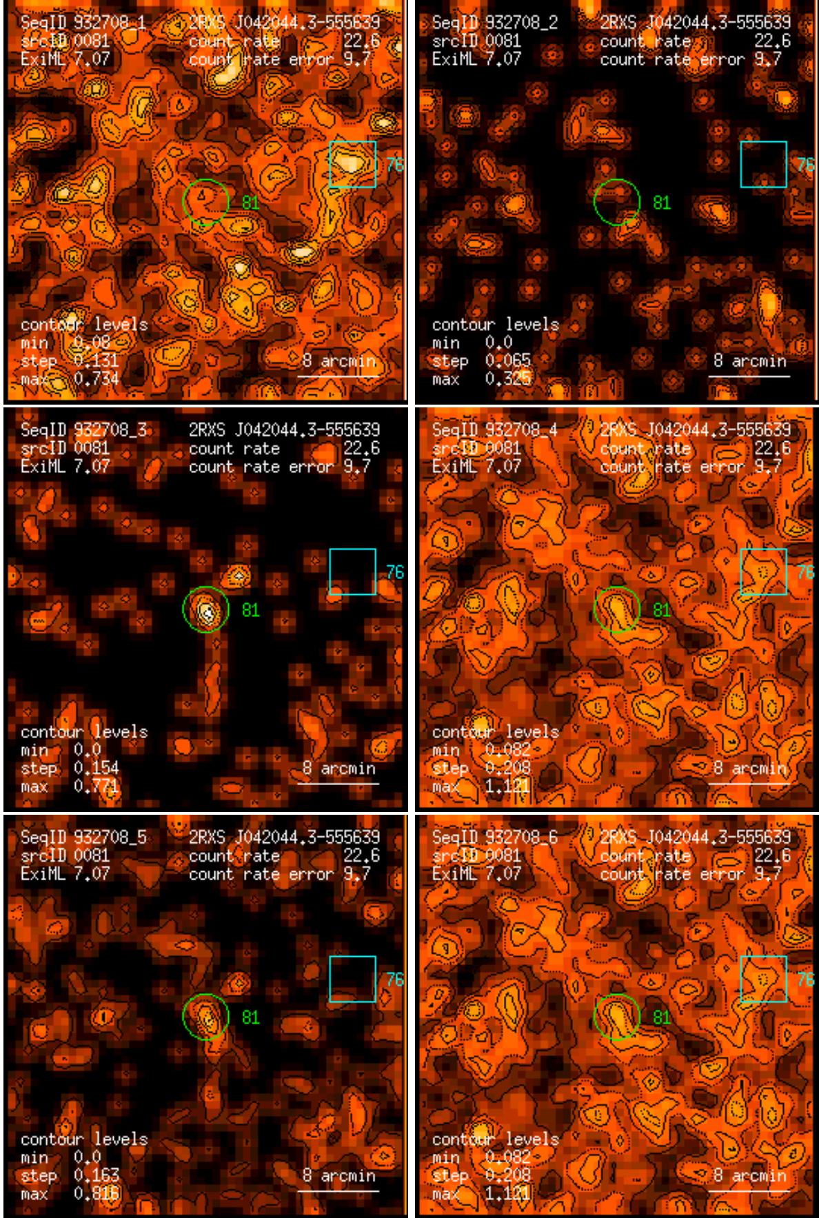
Figure 81: RASS 932708: detection 0081: band rate images, Gaussian filter: (1) PSPC channels 11 – 41, (2) 52 – 90, (3) 91 – 201, (4) 11 – 235, (5) 52 – 201, (6) 11 – 201. Broad band rates in counts/ks. Band rate contour levels in counts/ks/arcmin 2 .
