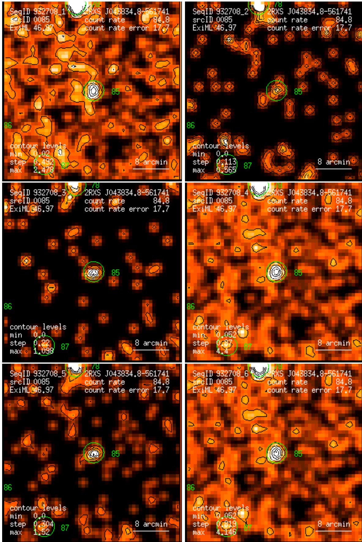
Figure 85: RASS 932708: detection 0085: band rate images, Gaussian filter: (1) PSPC channels 11 – 41, (2) 52 – 90, (3) 91 – 201, (4) 11 – 235, (5) 52 – 201, (6) 11 – 201. Broad band rates in counts/ks. Band rate contour levels in counts/ks/arcmin 2 .
