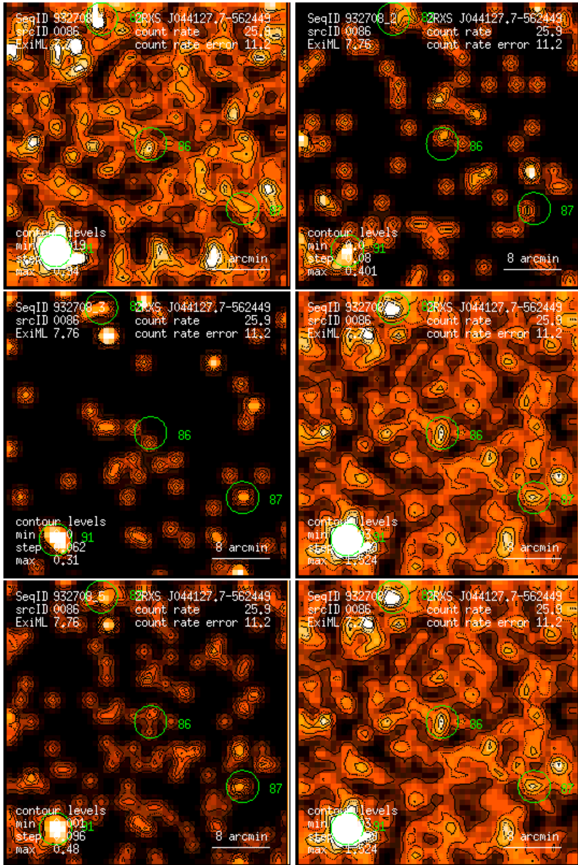
Figure 86: RASS 932708: detection 0086: band rate images, Gaussian filter: (1) PSPC channels 11 – 41, (2) 52 – 90, (3) 91 – 201, (4) 11 – 235, (5) 52 – 201, (6) 11 – 201. Broad band rates in counts/ks. Band rate contour levels in counts/ks/arcmin 2 .
