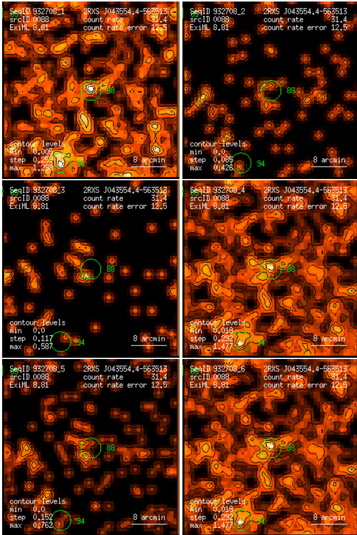
Figure 88: RASS 932708: detection 0088: band rate images, Gaussian filter: (1) PSPC channels 11 – 41, (2) 52 – 90, (3) 91 – 201, (4) 11 – 235, (5) 52 – 201, (6) 11 – 201. Broad band rates in counts/ks. Band rate contour levels in counts/ks/arcmin 2 .
