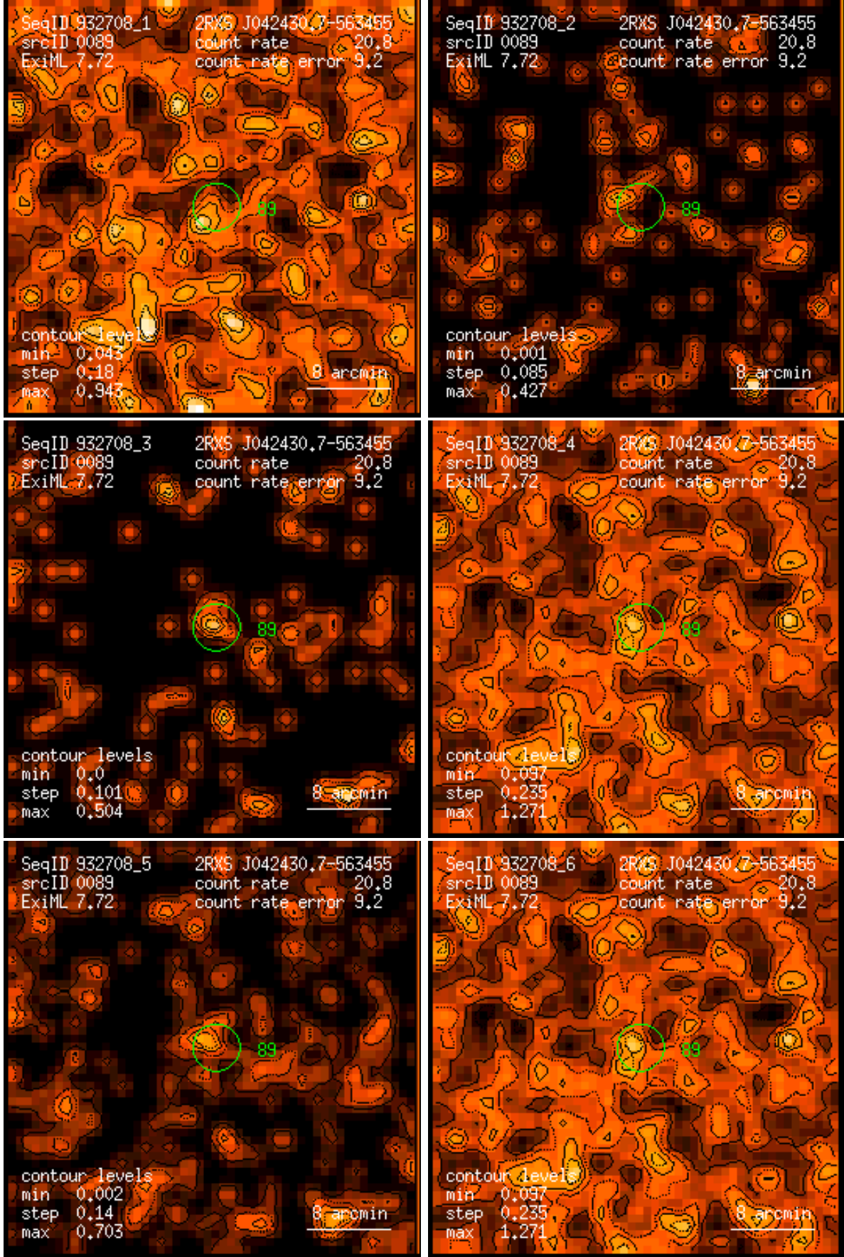
Figure 89: RASS 932708: detection 0089: band rate images, Gaussian filter: (1) PSPC channels 11 – 41, (2) 52 – 90, (3) 91 – 201, (4) 11 – 235, (5) 52 – 201, (6) 11 – 201. Broad band rates in counts/ks. Band rate contour levels in counts/ks/arcmin 2 .
