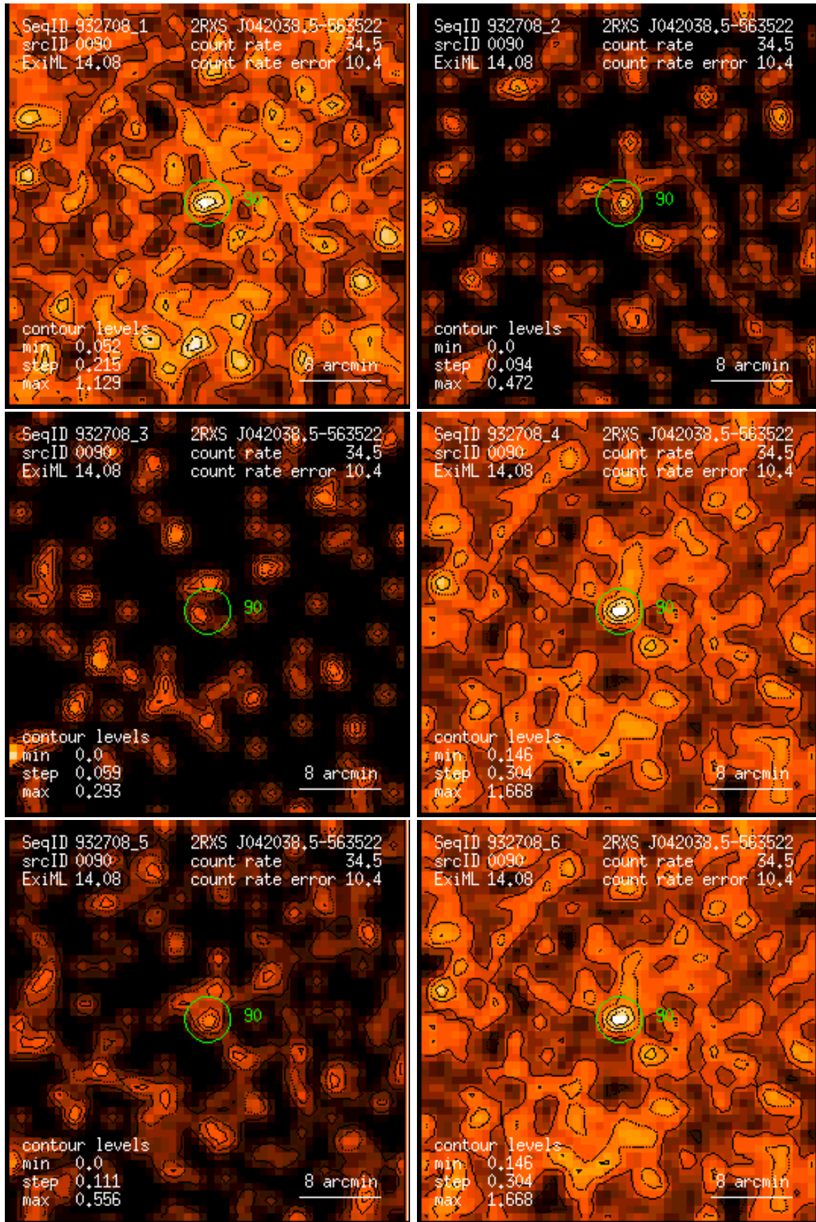
Figure 90: RASS 932708: detection 0090: band rate images, Gaussian filter: (1) PSPC channels 11 – 41, (2) 52 – 90, (3) 91 – 201, (4) 11 – 235, (5) 52 – 201, (6) 11 – 201. Broad band rates in counts/ks. Band rate contour levels in counts/ks/arcmin 2 .
