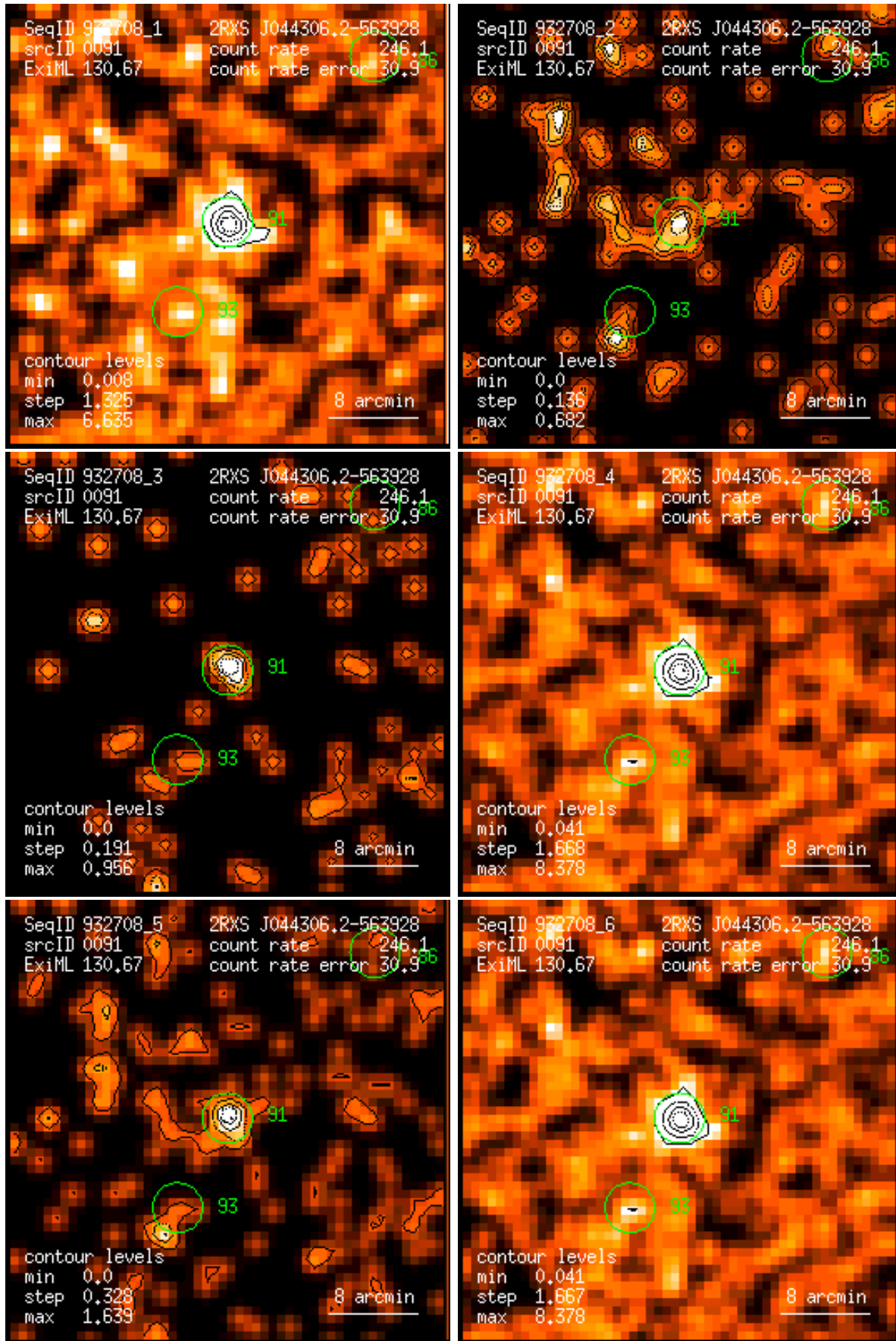
Figure 91: RASS 932708: detection 0091: band rate images, Gaussian filter: (1) PSPC channels 11 – 41, (2) 52 – 90, (3) 91 – 201, (4) 11 – 235, (5) 52 – 201, (6) 11 – 201. Broad band rates in counts/ks. Band rate contour levels in counts/ks/arcmin 2 .
