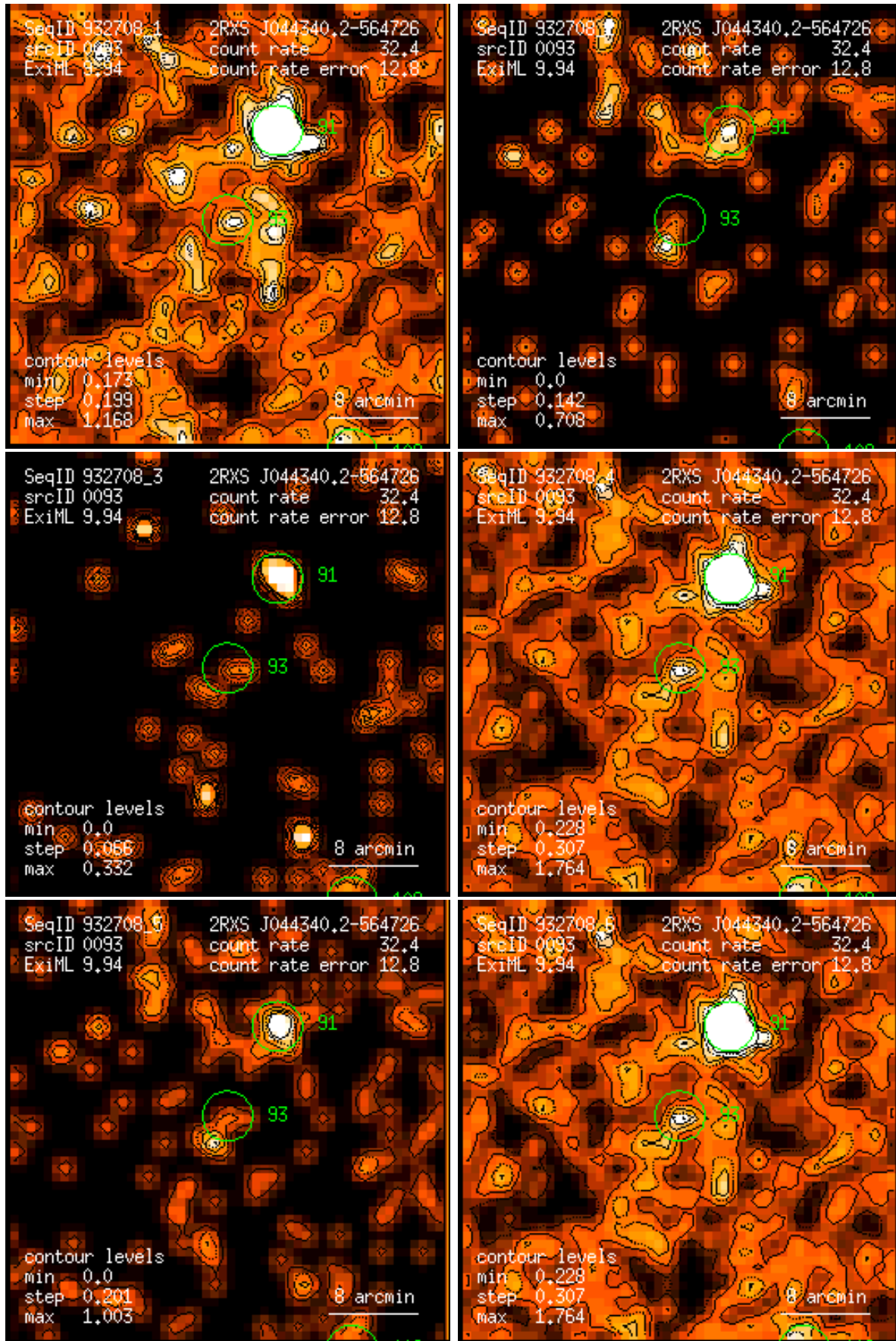
Figure 93: RASS 932708: detection 0093: band rate images, Gaussian filter: (1) PSPC channels 11 – 41, (2) 52 – 90, (3) 91 – 201, (4) 11 – 235, (5) 52 – 201, (6) 11 – 201. Broad band rates in counts/ks. Band rate contour levels in counts/ks/arcmin 2 .
