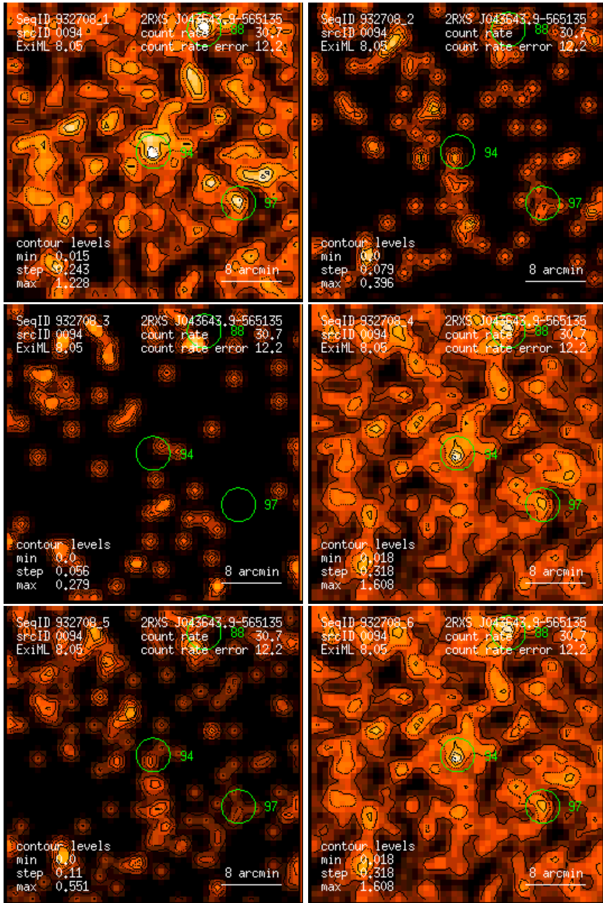
Figure 94: RASS 932708: detection 0094: band rate images, Gaussian filter: (1) PSPC channels 11 – 41, (2) 52 – 90, (3) 91 – 201, (4) 11 – 235, (5) 52 – 201, (6) 11 – 201. Broad band rates in counts/ks. Band rate contour levels in counts/ks/arcmin 2 .
