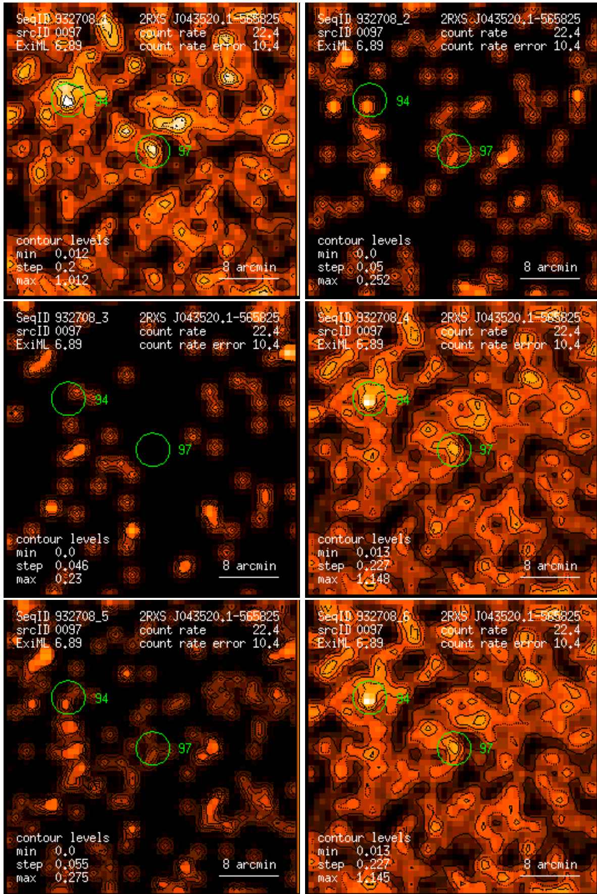
Figure 97: RASS 932708: detection 0097: band rate images, Gaussian filter: (1) PSPC channels 11 – 41, (2) 52 – 90, (3) 91 – 201, (4) 11 – 235, (5) 52 – 201, (6) 11 – 201. Broad band rates in counts/ks. Band rate contour levels in counts/ks/arcmin 2 .
