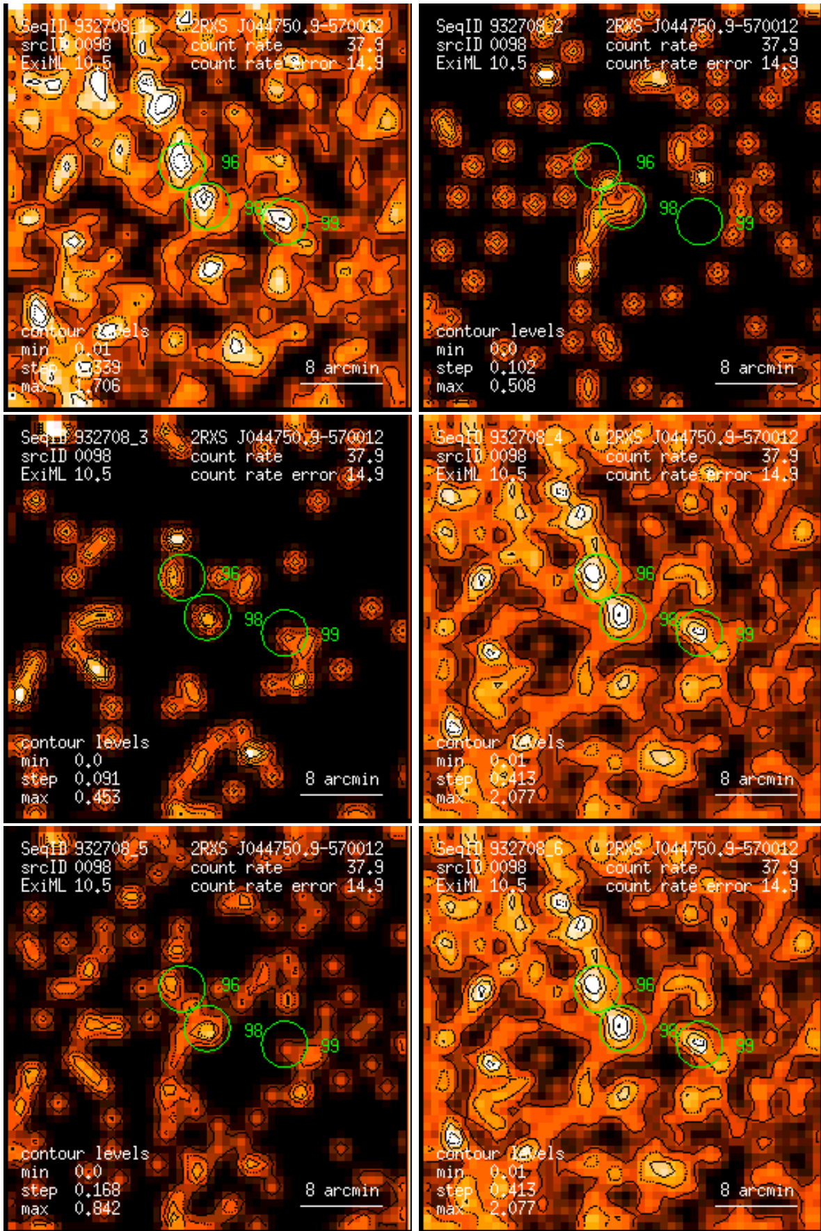
Figure 98: RASS 932708: detection 0098: band rate images, Gaussian filter: (1) PSPC channels 11 – 41, (2) 52 – 90, (3) 91 – 201, (4) 11 – 235, (5) 52 – 201, (6) 11 – 201. Broad band rates in counts/ks. Band rate contour levels in counts/ks/arcmin 2 .
