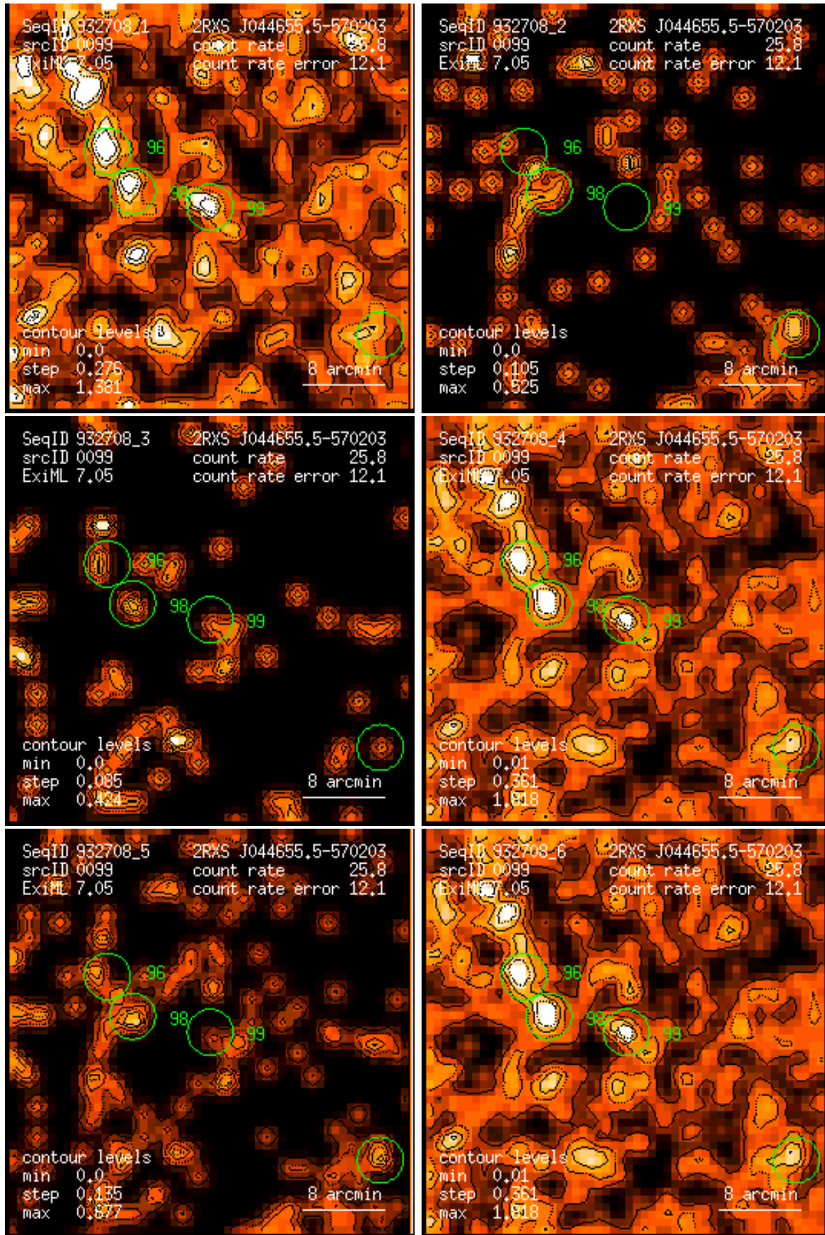
Figure 99: RASS 932708: detection 0099: band rate images, Gaussian filter: (1) PSPC channels 11 – 41, (2) 52 – 90, (3) 91 – 201, (4) 11 – 235, (5) 52 – 201, (6) 11 – 201. Broad band rates in counts/ks. Band rate contour levels in counts/ks/arcmin 2 .
