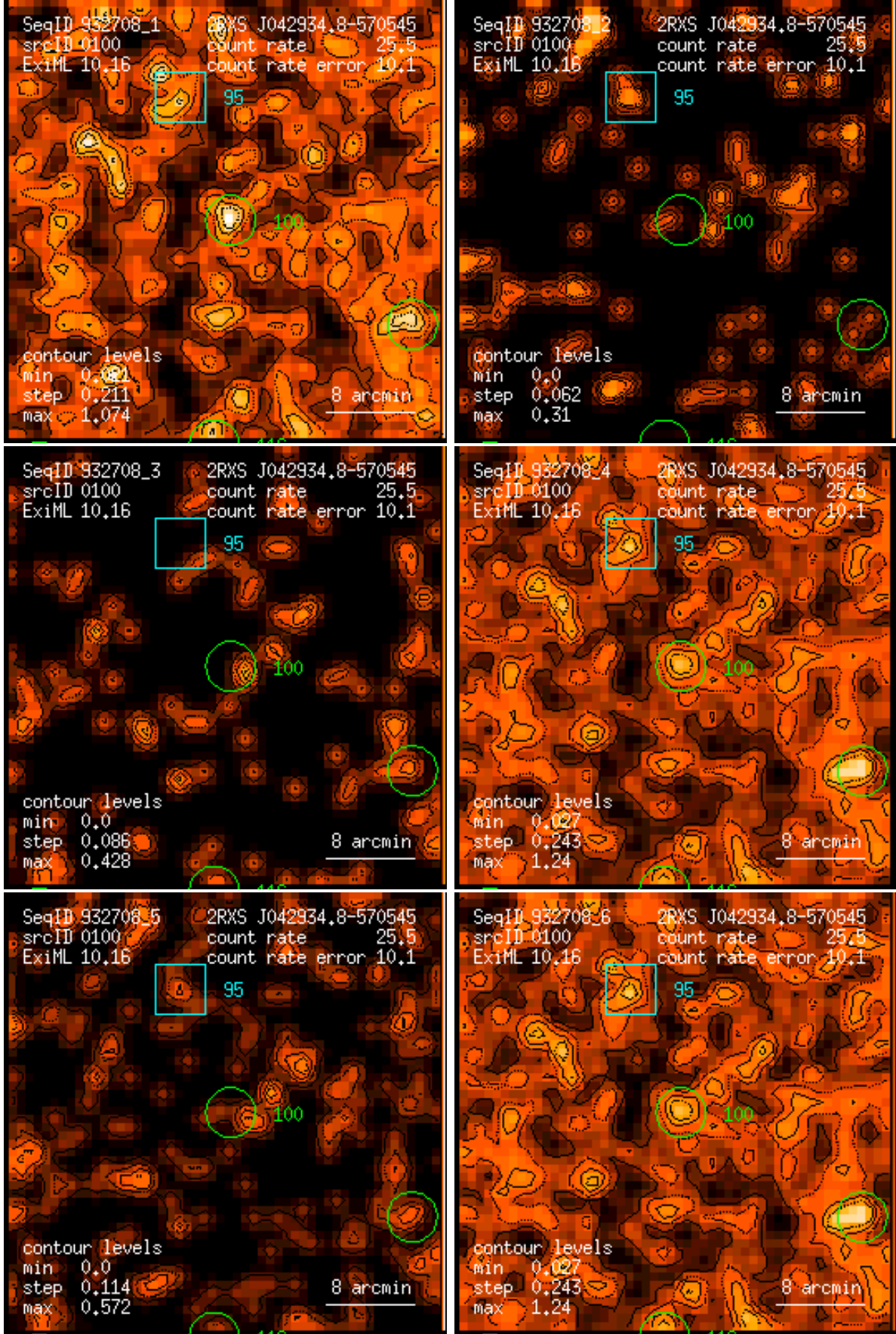
Figure 100: RASS 932708: detection 0100: band rate images, Gaussian filter: (1) PSPC channels 11 – 41, (2) 52 – 90, (3) 91 – 201, (4) 11 – 235, (5) 52 – 201, (6) 11 – 201. Broad band rates in counts/ks. Band rate contour levels in counts/ks/arcmin 2 .
