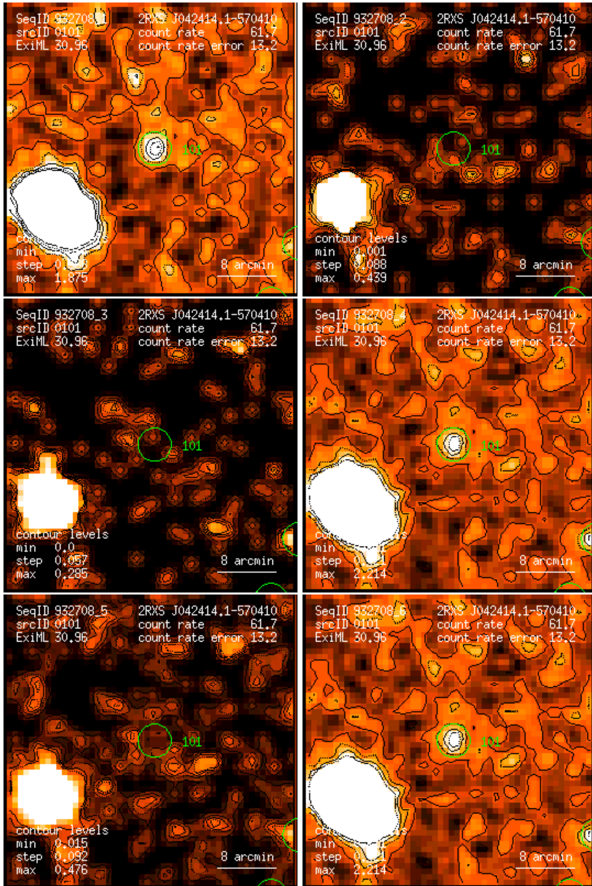
Figure 101: RASS 932708: detection 0101: band rate images, Gaussian filter: (1) PSPC channels 11 – 41, (2) 52 – 90, (3) 91 – 201, (4) 11 – 235, (5) 52 – 201, (6) 11 – 201. Broad band rates in counts/ks. Band rate contour levels in counts/ks/arcmin 2 .
