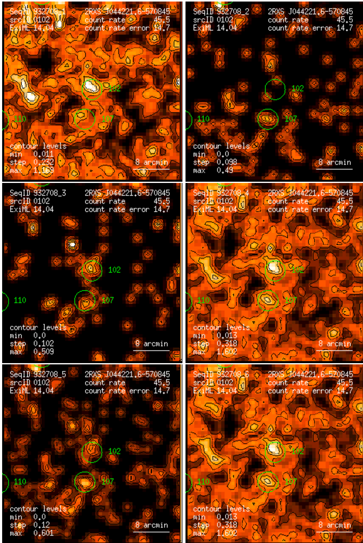
Figure 102: RASS 932708: detection 0102: band rate images, Gaussian filter: (1) PSPC channels 11 – 41, (2) 52 – 90, (3) 91 – 201, (4) 11 – 235, (5) 52 – 201, (6) 11 – 201. Broad band rates in counts/ks. Band rate contour levels in counts/ks/arcmin 2 .
