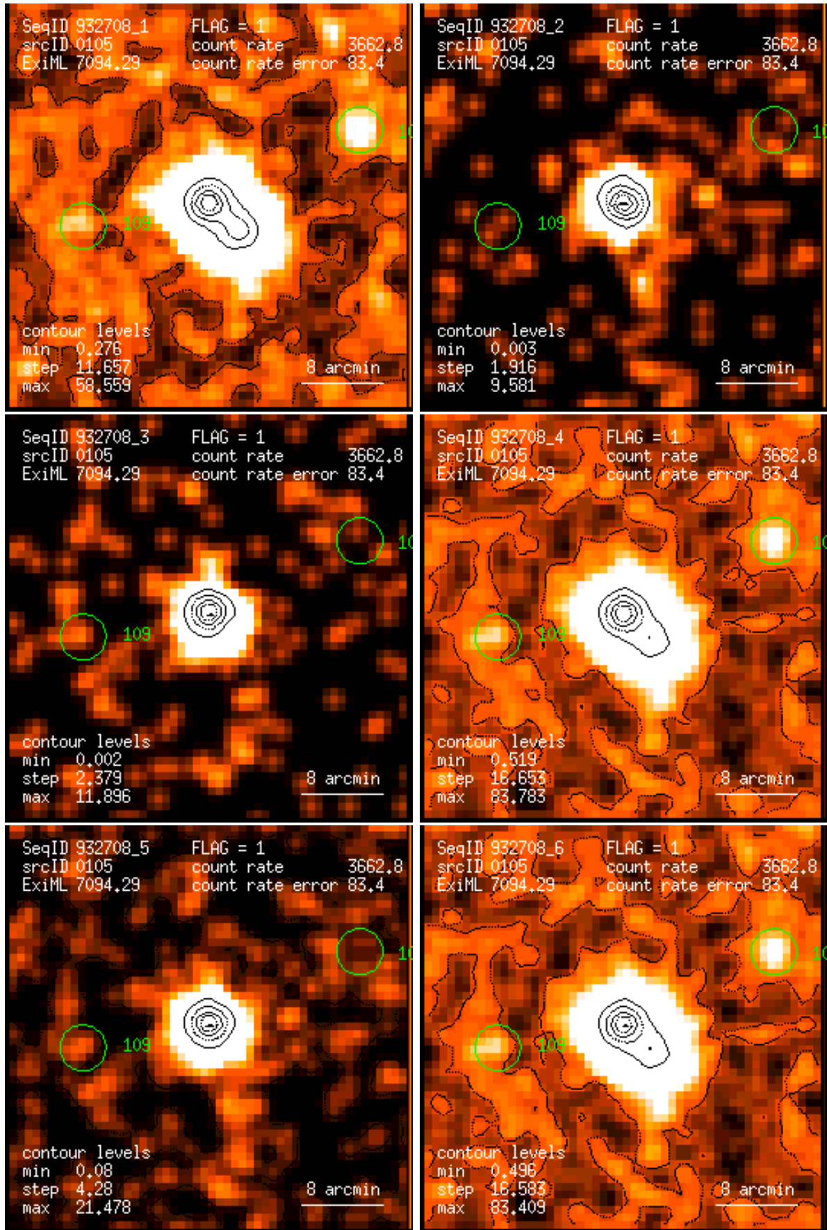
Figure 105: RASS 932708: detection 0105: band rate images, Gaussian filter: (1) PSPC channels 11 – 41, (2) 52 – 90, (3) 91 – 201, (4) 11 – 235, (5) 52 – 201, (6) 11 – 201. Broad band rates in counts/ks. Band rate contour levels in counts/ks/arcmin 2 .
