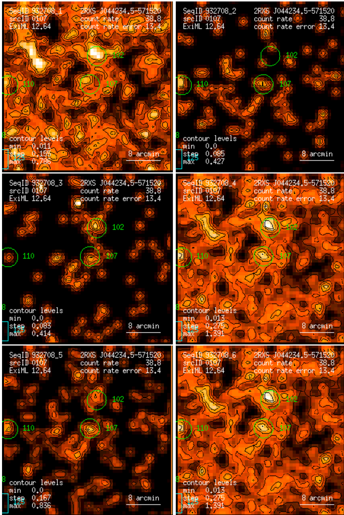
Figure 107: RASS 932708: detection 0107: band rate images, Gaussian filter: (1) PSPC channels 11 – 41, (2) 52 – 90, (3) 91 – 201, (4) 11 – 235, (5) 52 – 201, (6) 11 – 201. Broad band rates in counts/ks. Band rate contour levels in counts/ks/arcmin 2 .
