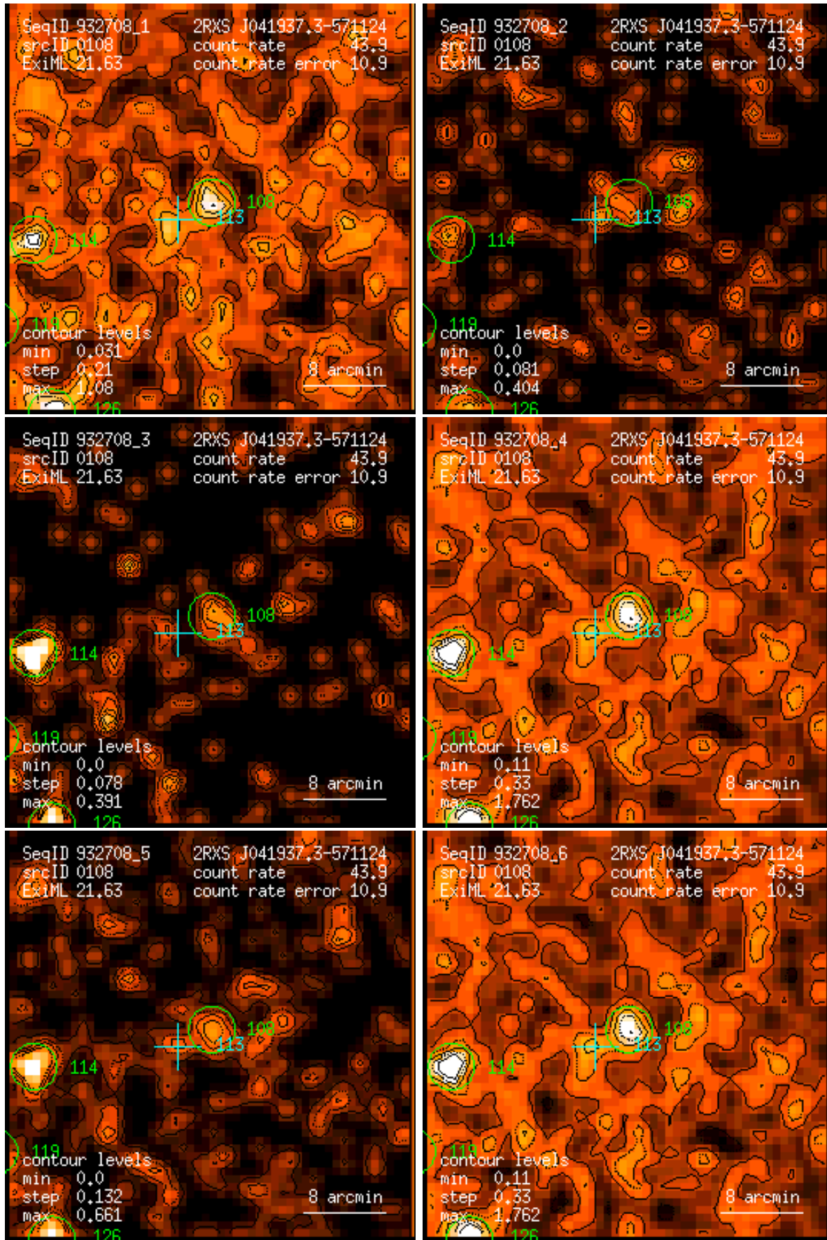
Figure 108: RASS 932708: detection 0108: band rate images, Gaussian filter: (1) PSPC channels 11 – 41, (2) 52 – 90, (3) 91 – 201, (4) 11 – 235, (5) 52 – 201, (6) 11 – 201. Broad band rates in counts/ks. Band rate contour levels in counts/ks/arcmin 2 .
