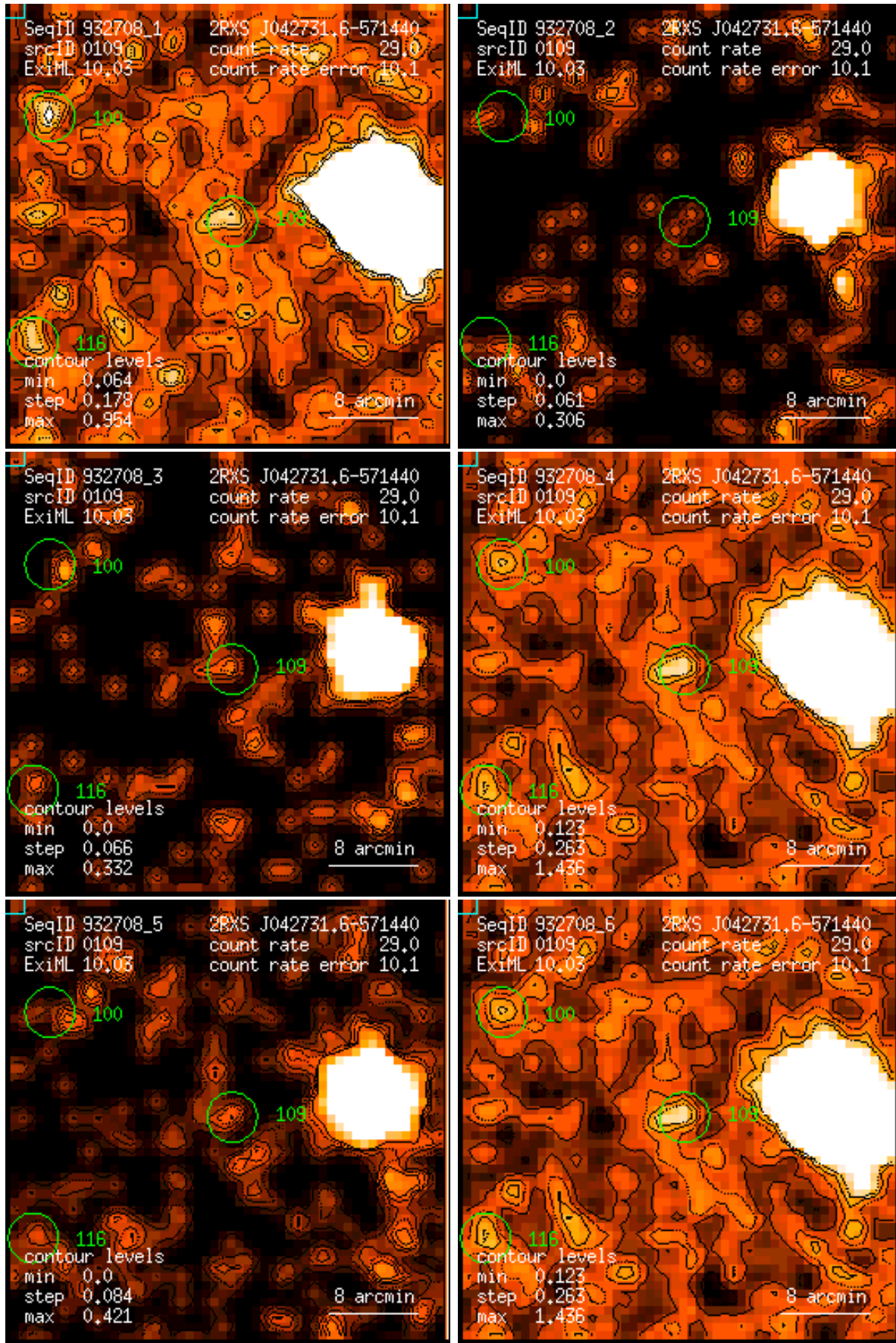
Figure 109: RASS 932708: detection 0109: band rate images, Gaussian filter: (1) PSPC channels 11 – 41, (2) 52 – 90, (3) 91 – 201, (4) 11 – 235, (5) 52 – 201, (6) 11 – 201. Broad band rates in counts/ks. Band rate contour levels in counts/ks/arcmin 2 .
