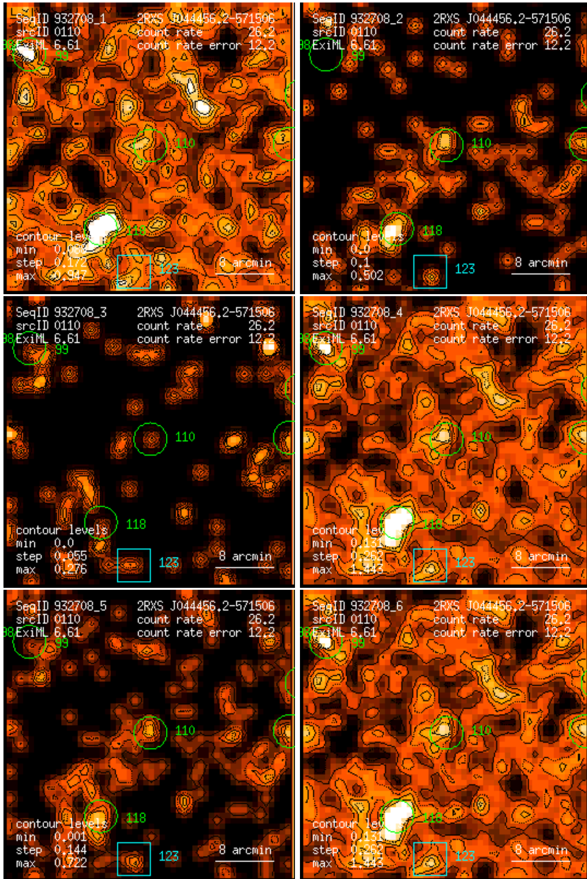
Figure 110: RASS 932708: detection 0110: band rate images, Gaussian filter: (1) PSPC channels 11 – 41, (2) 52 – 90, (3) 91 – 201, (4) 11 – 235, (5) 52 – 201, (6) 11 – 201. Broad band rates in counts/ks. Band rate contour levels in counts/ks/arcmin 2 .
