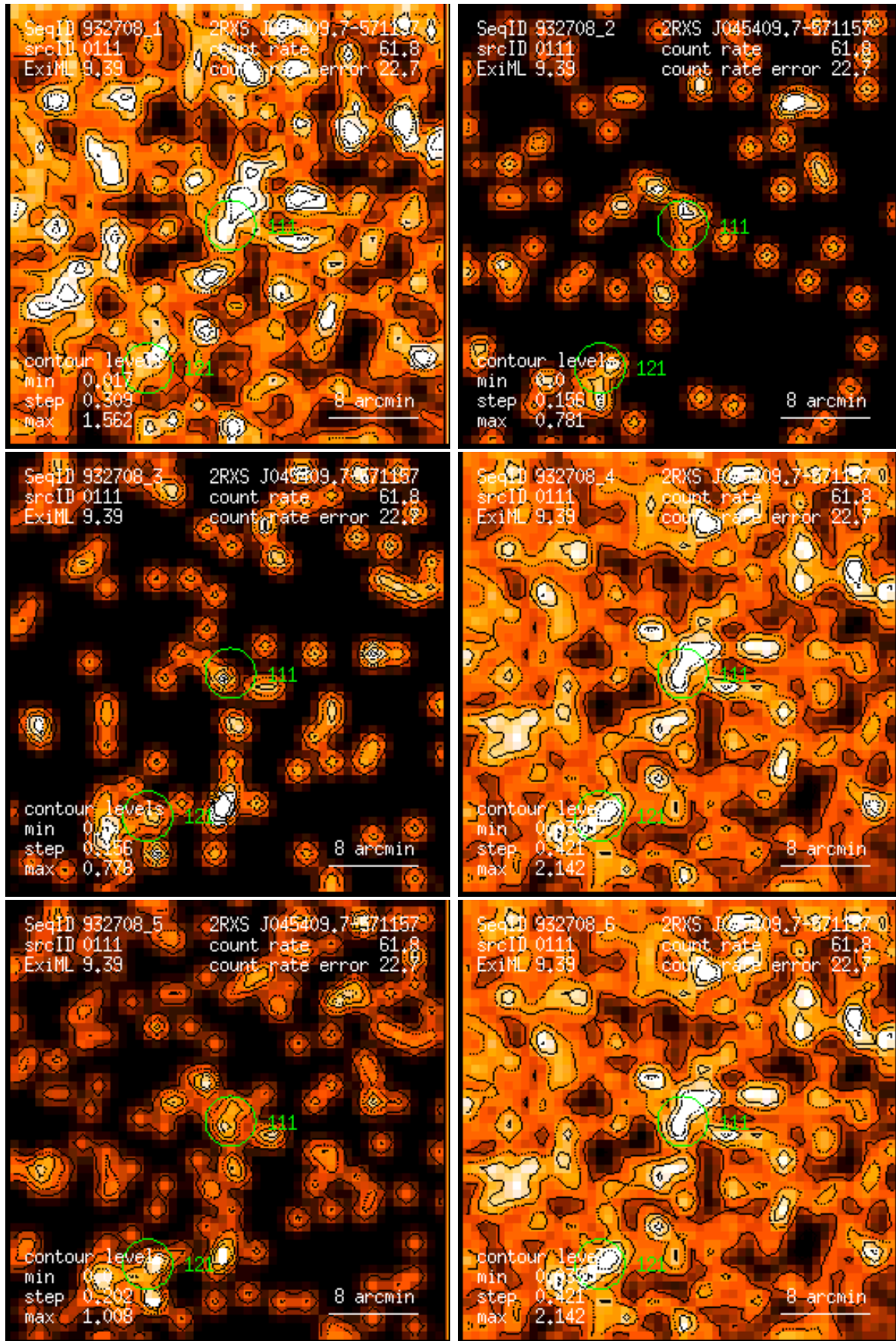
Figure 111: RASS 932708: detection 0111: band rate images, Gaussian filter: (1) PSPC channels 11 – 41, (2) 52 – 90, (3) 91 – 201, (4) 11 – 235, (5) 52 – 201, (6) 11 – 201. Broad band rates in counts/ks. Band rate contour levels in counts/ks/arcmin 2 .
