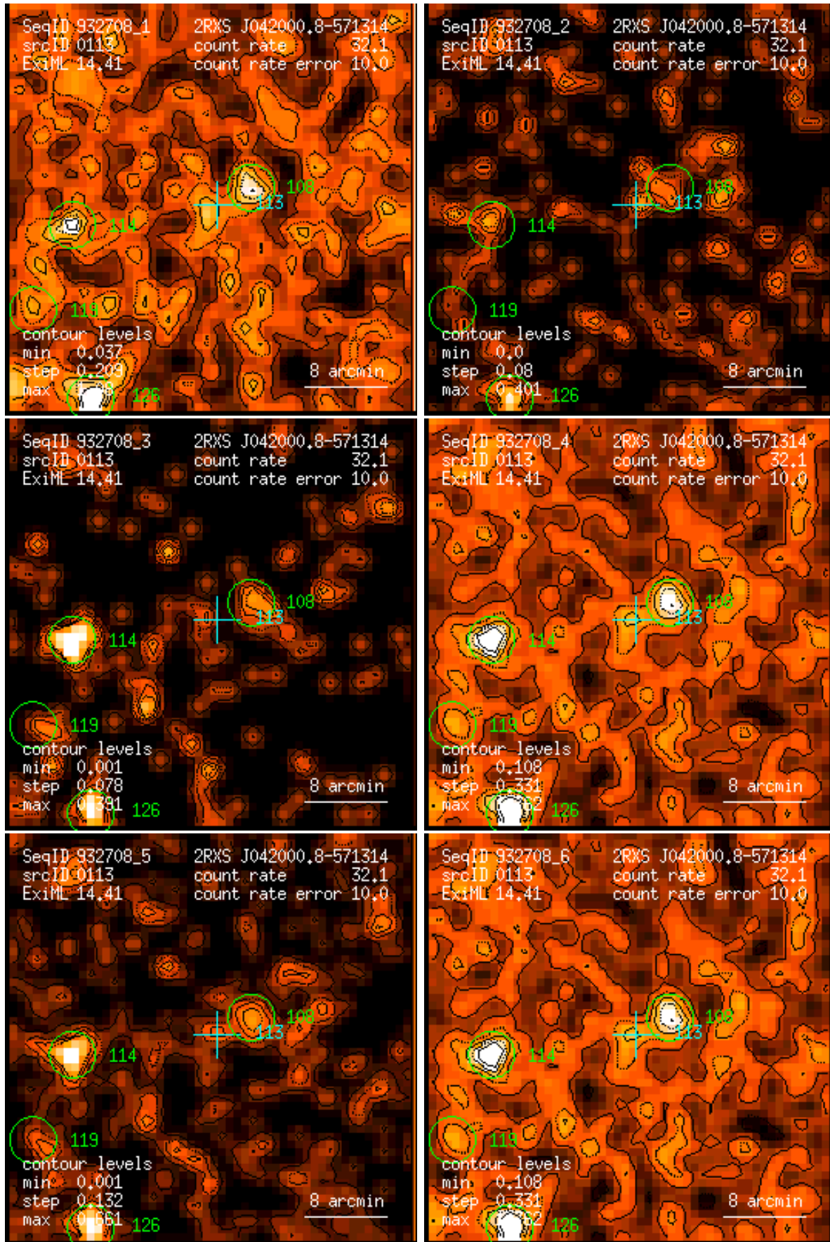
Figure 113: RASS 932708: detection 0113: band rate images, Gaussian filter: (1) PSPC channels 11 – 41, (2) 52 – 90, (3) 91 – 201, (4) 11 – 235, (5) 52 – 201, (6) 11 – 201. Broad band rates in counts/ks. Band rate contour levels in counts/ks/arcmin 2 .
