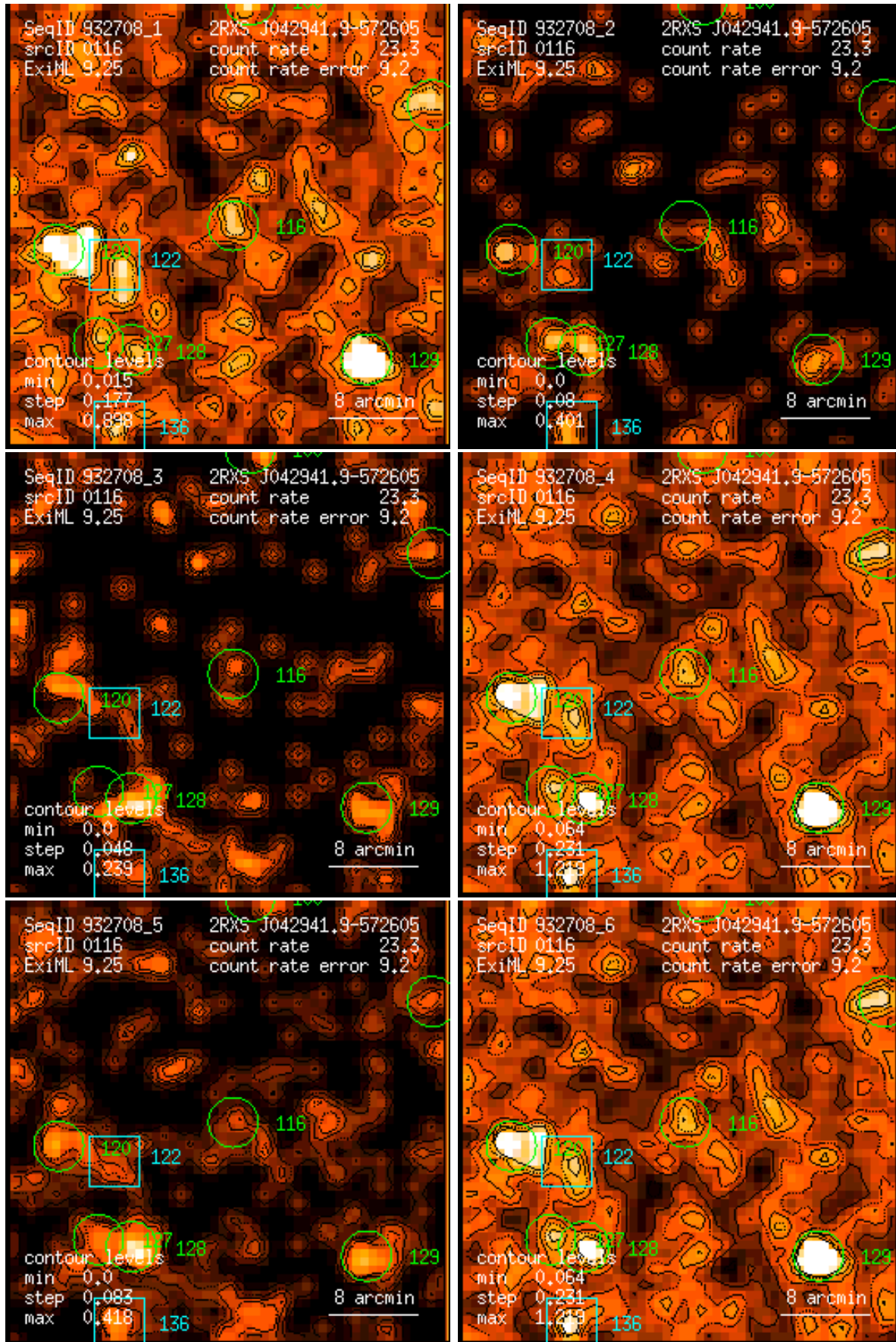
Figure 116: RASS 932708: detection 0116: band rate images, Gaussian filter: (1) PSPC channels 11 – 41, (2) 52 – 90, (3) 91 – 201, (4) 11 – 235, (5) 52 – 201, (6) 11 – 201. Broad band rates in counts/ks. Band rate contour levels in counts/ks/arcmin 2 .
