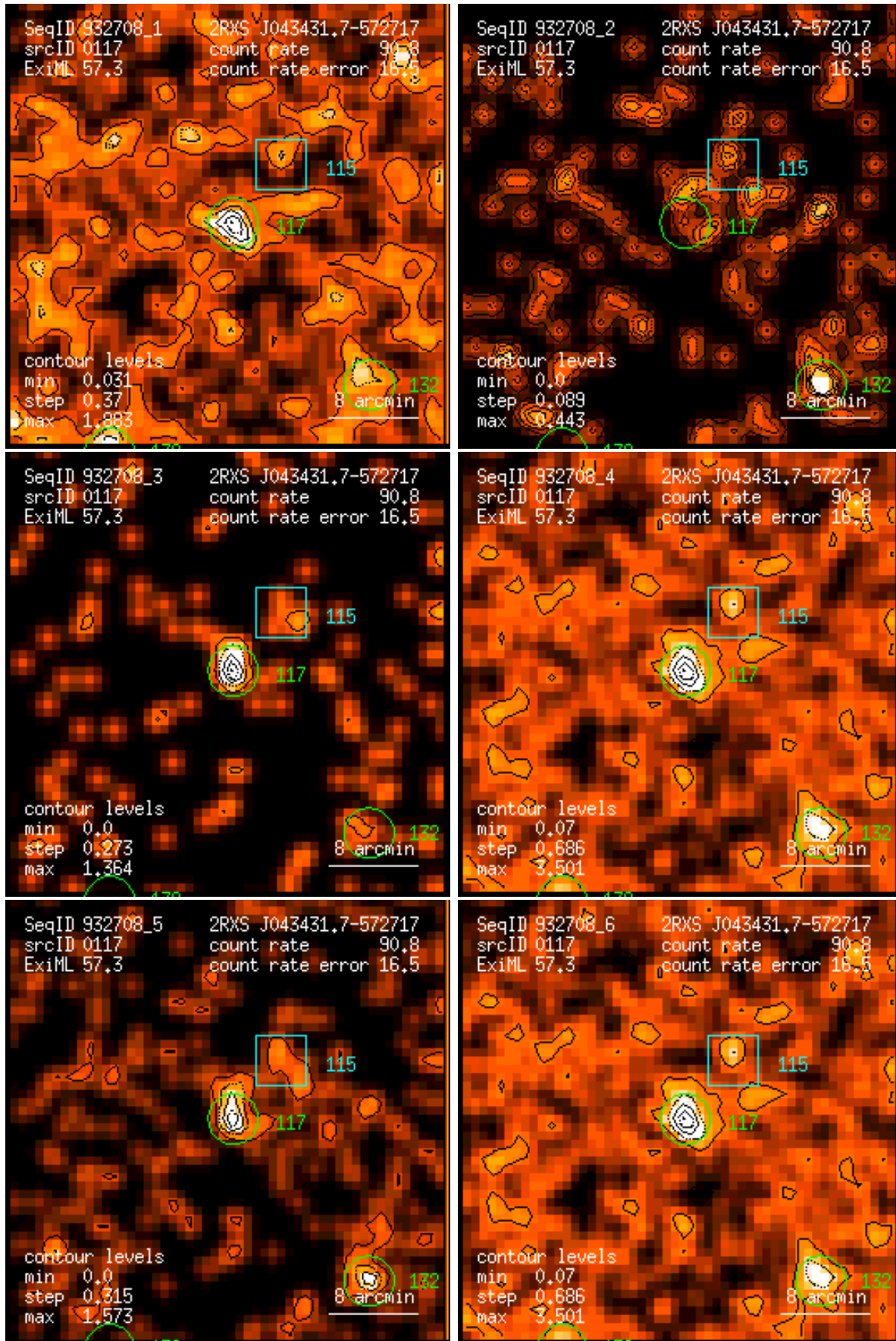
Figure 117: RASS 932708: detection 0117: band rate images, Gaussian filter: (1) PSPC channels 11 – 41, (2) 52 – 90, (3) 91 – 201, (4) 11 – 235, (5) 52 – 201, (6) 11 – 201. Broad band rates in counts/ks. Band rate contour levels in counts/ks/arcmin 2 .
