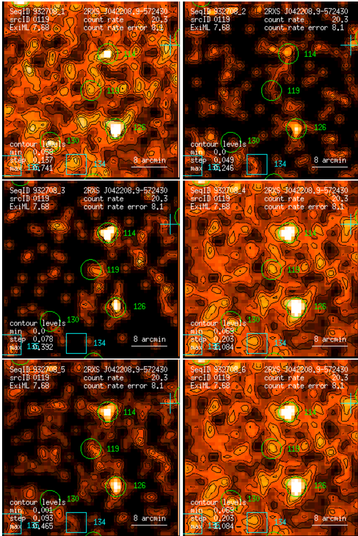
Figure 119: RASS 932708: detection 0119: band rate images, Gaussian filter: (1) PSPC channels 11 – 41, (2) 52 – 90, (3) 91 – 201, (4) 11 – 235, (5) 52 – 201, (6) 11 – 201. Broad band rates in counts/ks. Band rate contour levels in counts/ks/arcmin 2 .
