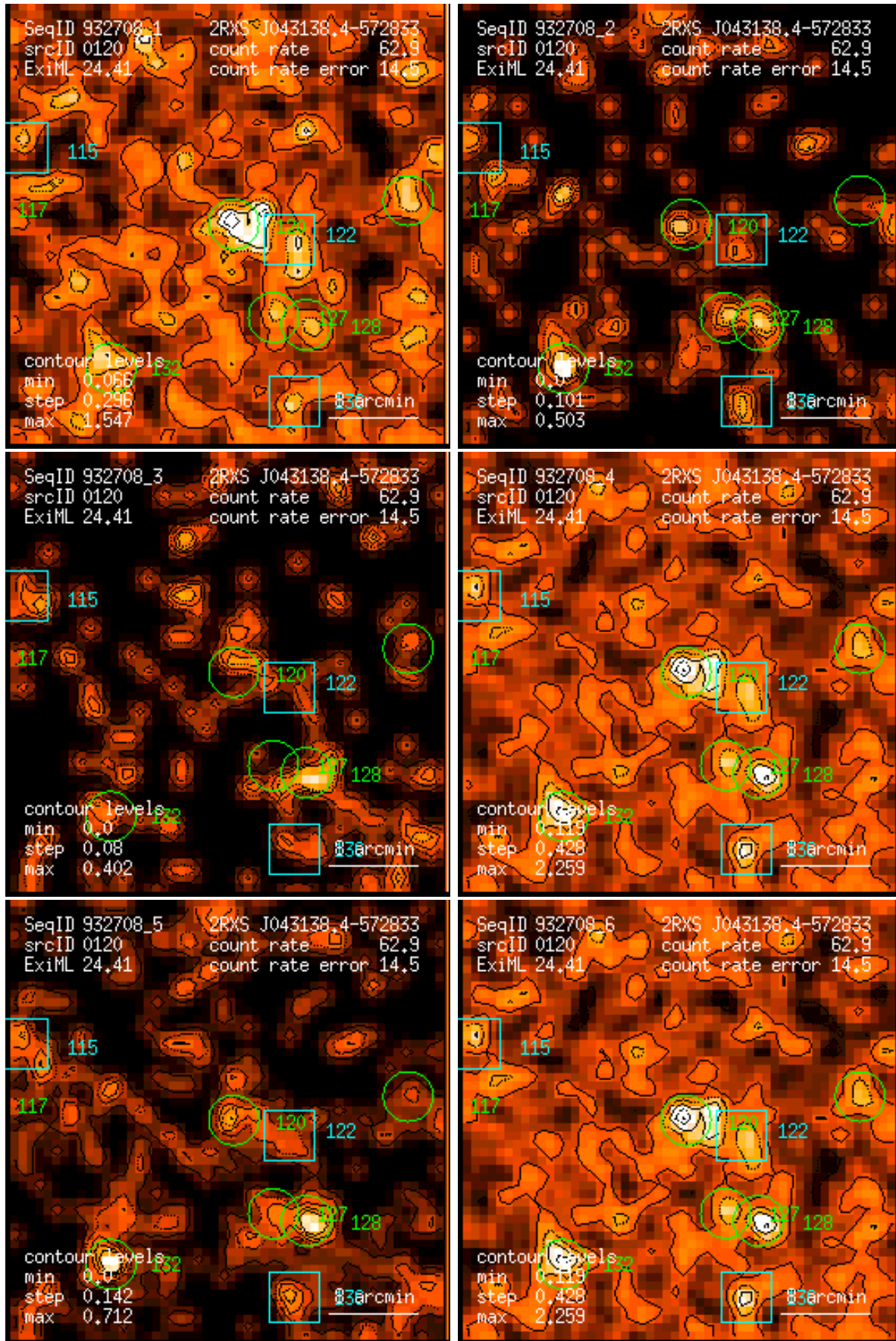
Figure 120: RASS 932708: detection 0120: band rate images, Gaussian filter: (1) PSPC channels 11 – 41, (2) 52 – 90, (3) 91 – 201, (4) 11 – 235, (5) 52 – 201, (6) 11 – 201. Broad band rates in counts/ks. Band rate contour levels in counts/ks/arcmin 2 .
