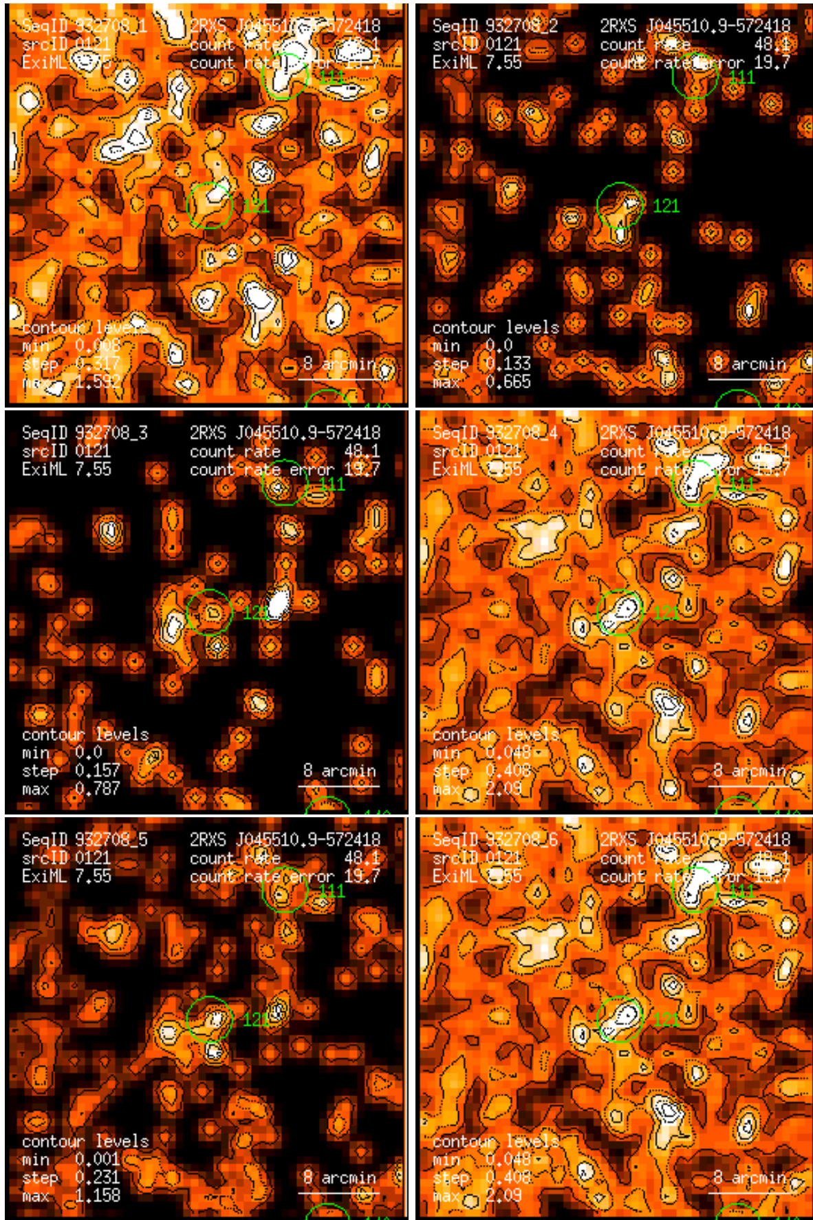
Figure 121: RASS 932708: detection 0121: band rate images, Gaussian filter: (1) PSPC channels 11 – 41, (2) 52 – 90, (3) 91 – 201, (4) 11 – 235, (5) 52 – 201, (6) 11 – 201. Broad band rates in counts/ks. Band rate contour levels in counts/ks/arcmin 2 .
