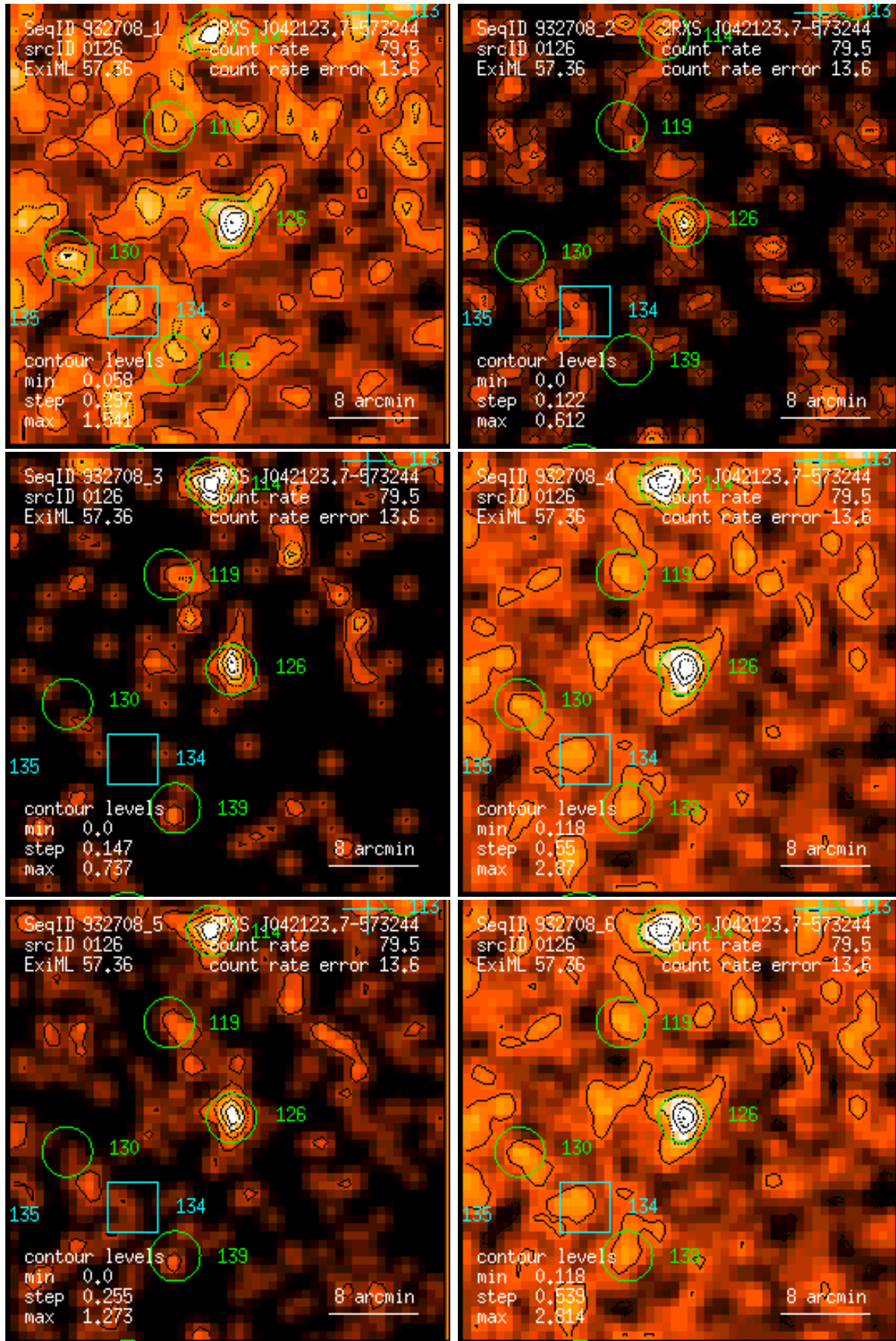
Figure 126: RASS 932708: detection 0126: band rate images, Gaussian filter: (1) PSPC channels 11 – 41, (2) 52 – 90, (3) 91 – 201, (4) 11 – 235, (5) 52 – 201, (6) 11 – 201. Broad band rates in counts/ks. Band rate contour levels in counts/ks/arcmin 2 .
