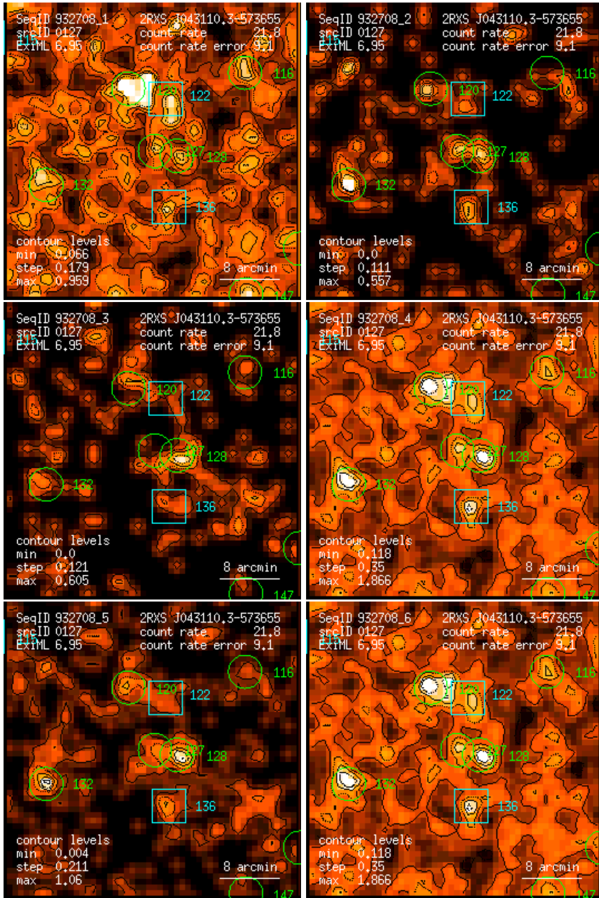
Figure 127: RASS 932708: detection 0127: band rate images, Gaussian filter: (1) PSPC channels 11 – 41, (2) 52 – 90, (3) 91 – 201, (4) 11 – 235, (5) 52 – 201, (6) 11 – 201. Broad band rates in counts/ks. Band rate contour levels in counts/ks/arcmin 2 .
