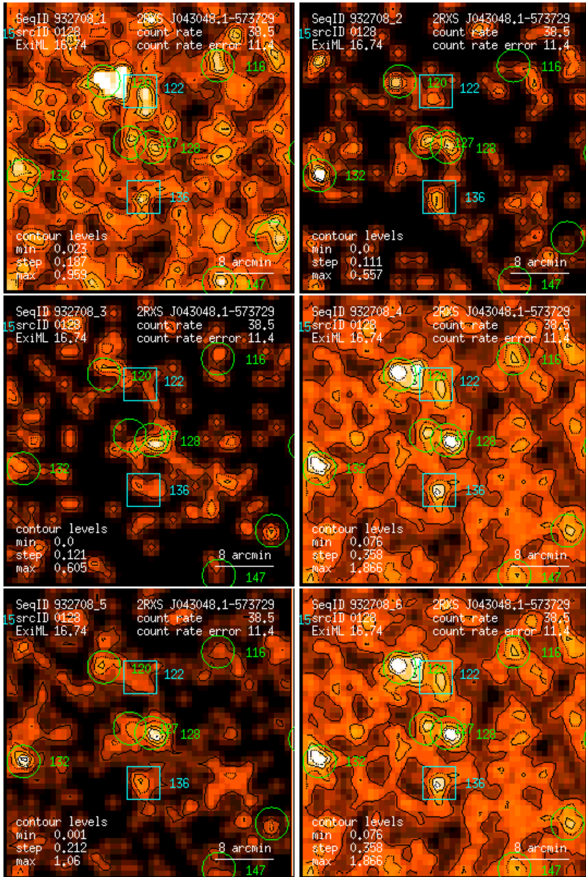
Figure 128: RASS 932708: detection 0128: band rate images, Gaussian filter: (1) PSPC channels 11 – 41, (2) 52 – 90, (3) 91 – 201, (4) 11 – 235, (5) 52 – 201, (6) 11 – 201. Broad band rates in counts/ks. Band rate contour levels in counts/ks/arcmin 2 .
