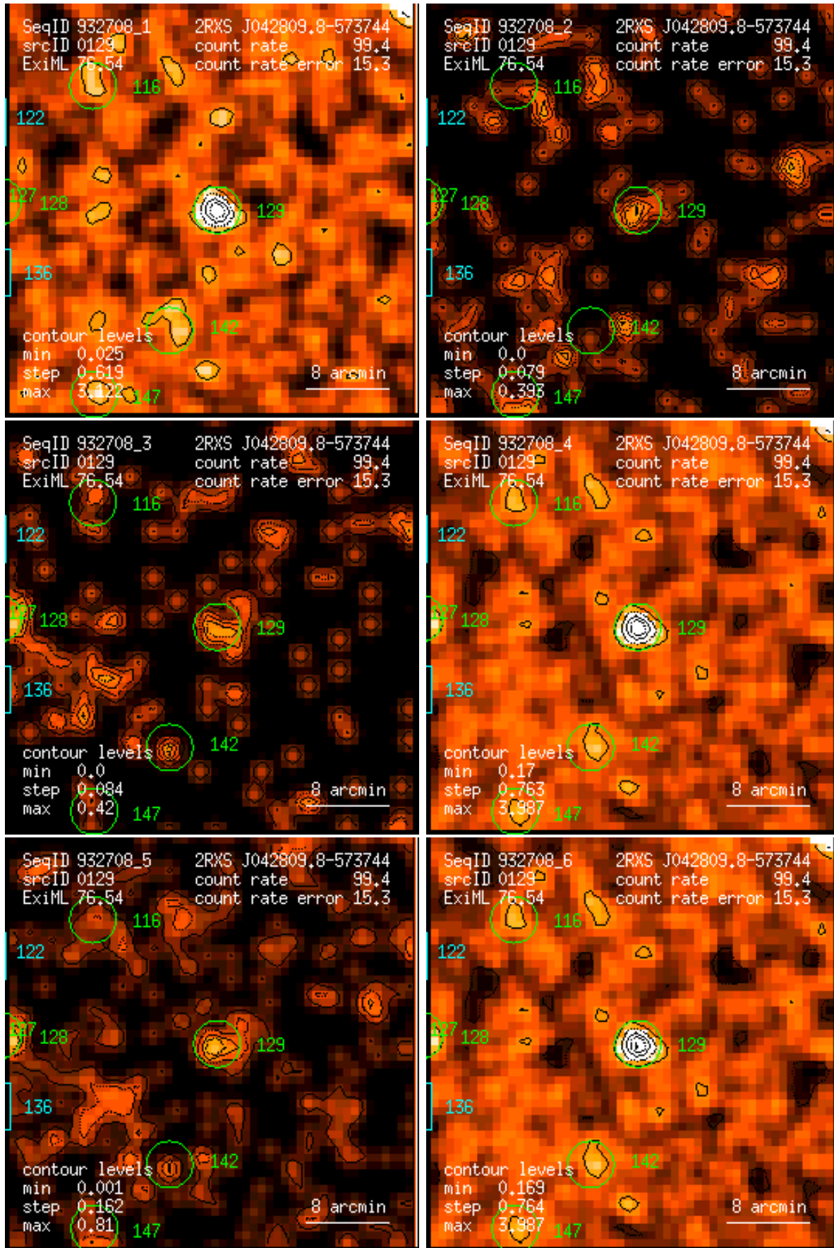
Figure 129: RASS 932708: detection 0129: band rate images, Gaussian filter: (1) PSPC channels 11 – 41, (2) 52 – 90, (3) 91 – 201, (4) 11 – 235, (5) 52 – 201, (6) 11 – 201. Broad band rates in counts/ks. Band rate contour levels in counts/ks/arcmin 2 .
