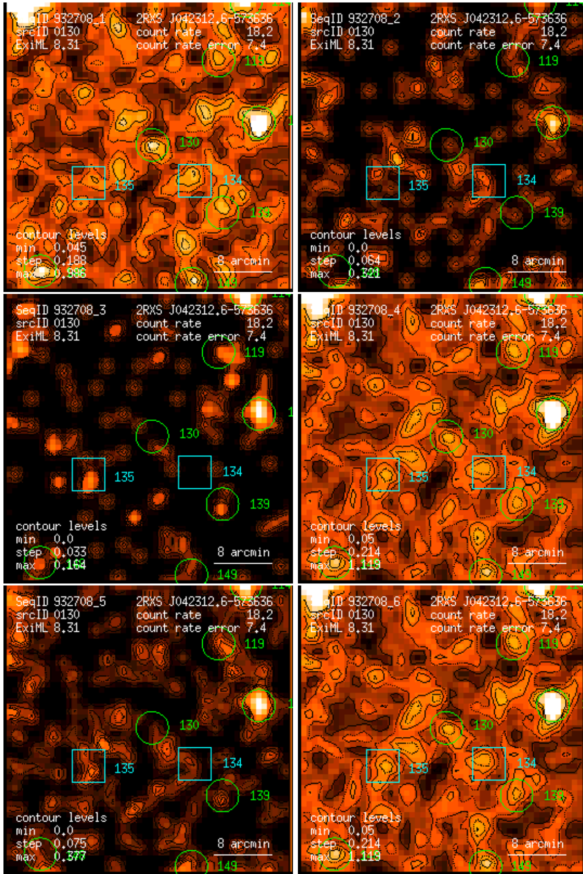
Figure 130: RASS 932708: detection 0130: band rate images, Gaussian filter: (1) PSPC channels 11 – 41, (2) 52 – 90, (3) 91 – 201, (4) 11 – 235, (5) 52 – 201, (6) 11 – 201. Broad band rates in counts/ks. Band rate contour levels in counts/ks/arcmin 2 .
