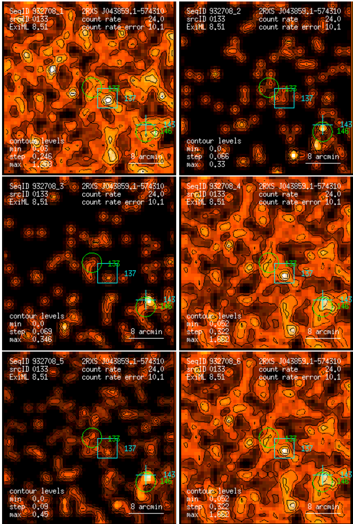
Figure 133: RASS 932708: detection 0133: band rate images, Gaussian filter: (1) PSPC channels 11 – 41, (2) 52 – 90, (3) 91 – 201, (4) 11 – 235, (5) 52 – 201, (6) 11 – 201. Broad band rates in counts/ks. Band rate contour levels in counts/ks/arcmin 2 .
