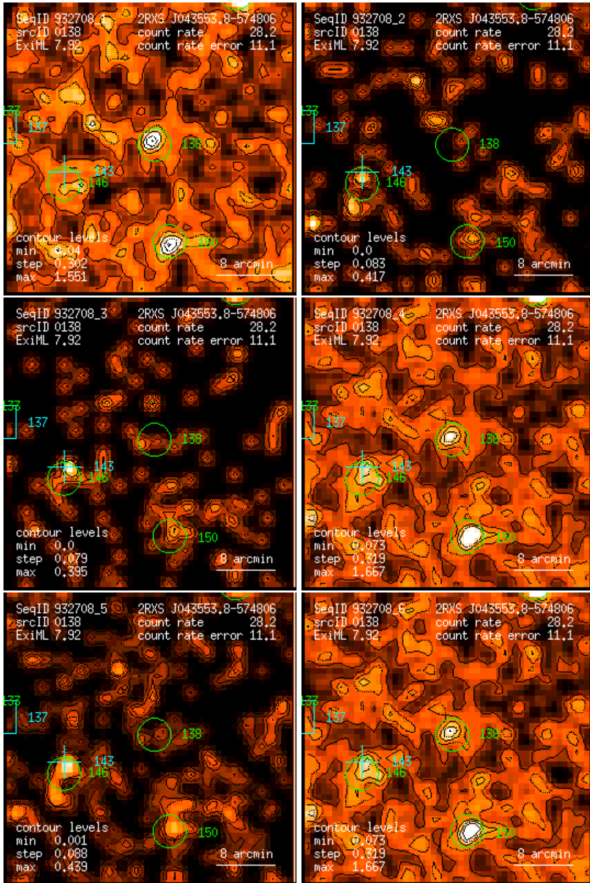
Figure 138: RASS 932708: detection 0138: band rate images, Gaussian filter: (1) PSPC channels 11 – 41, (2) 52 – 90, (3) 91 – 201, (4) 11 – 235, (5) 52 – 201, (6) 11 – 201. Broad band rates in counts/ks. Band rate contour levels in counts/ks/arcmin 2 .
