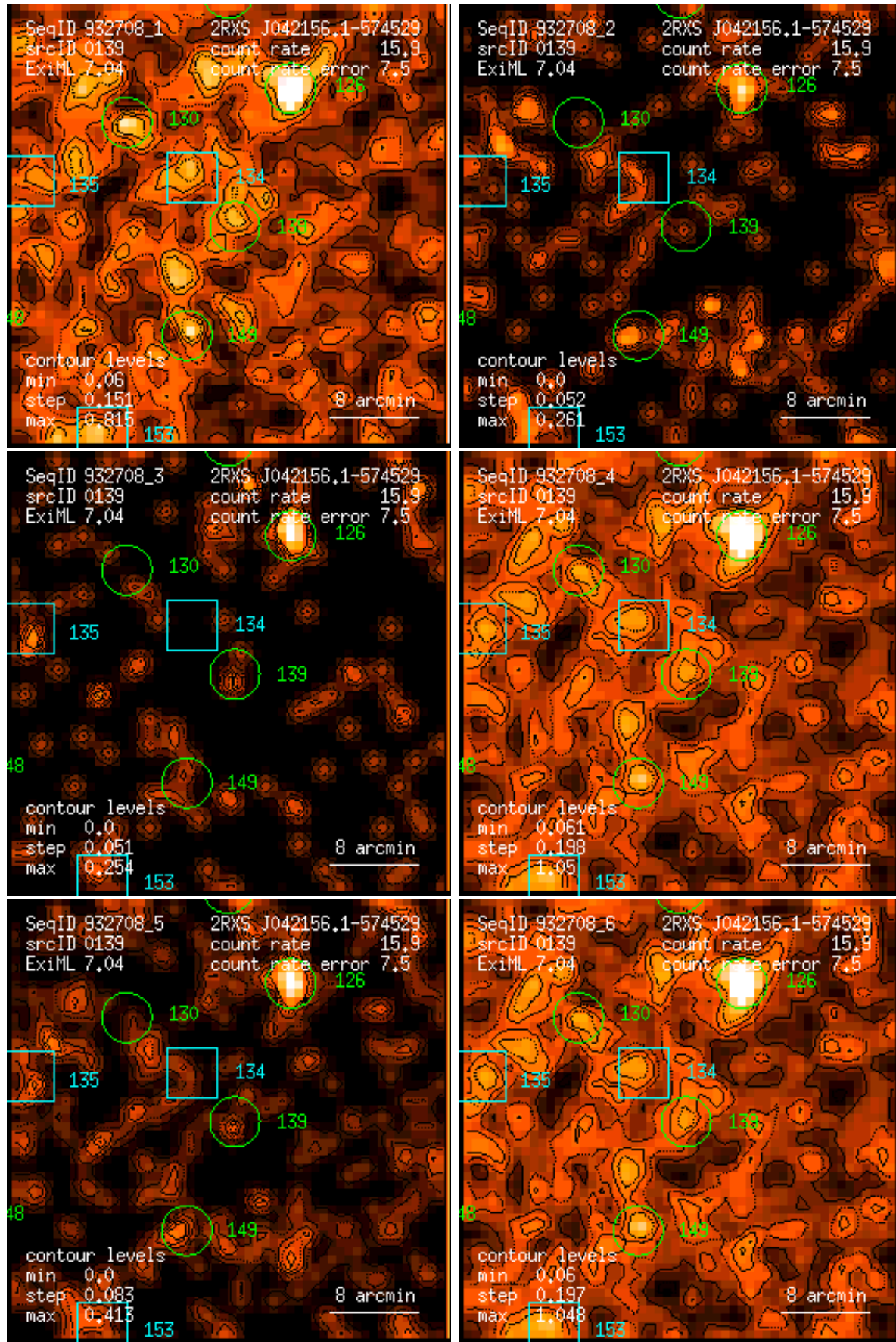
Figure 139: RASS 932708: detection 0139: band rate images, Gaussian filter: (1) PSPC channels 11 – 41, (2) 52 – 90, (3) 91 – 201, (4) 11 – 235, (5) 52 – 201, (6) 11 – 201. Broad band rates in counts/ks. Band rate contour levels in counts/ks/arcmin 2 .
