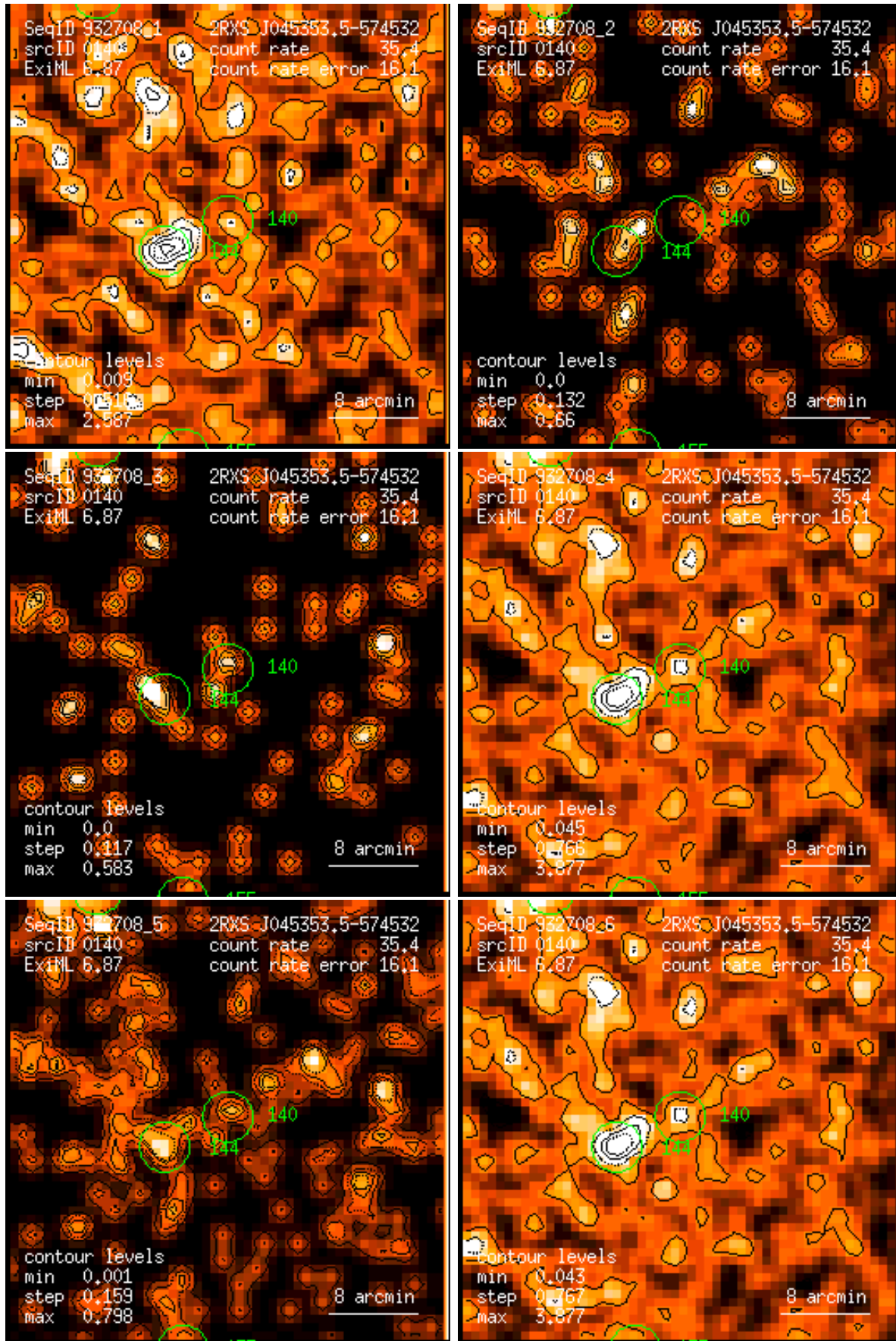
Figure 140: RASS 932708: detection 0140: band rate images, Gaussian filter: (1) PSPC channels 11 – 41, (2) 52 – 90, (3) 91 – 201, (4) 11 – 235, (5) 52 – 201, (6) 11 – 201. Broad band rates in counts/ks. Band rate contour levels in counts/ks/arcmin 2 .
