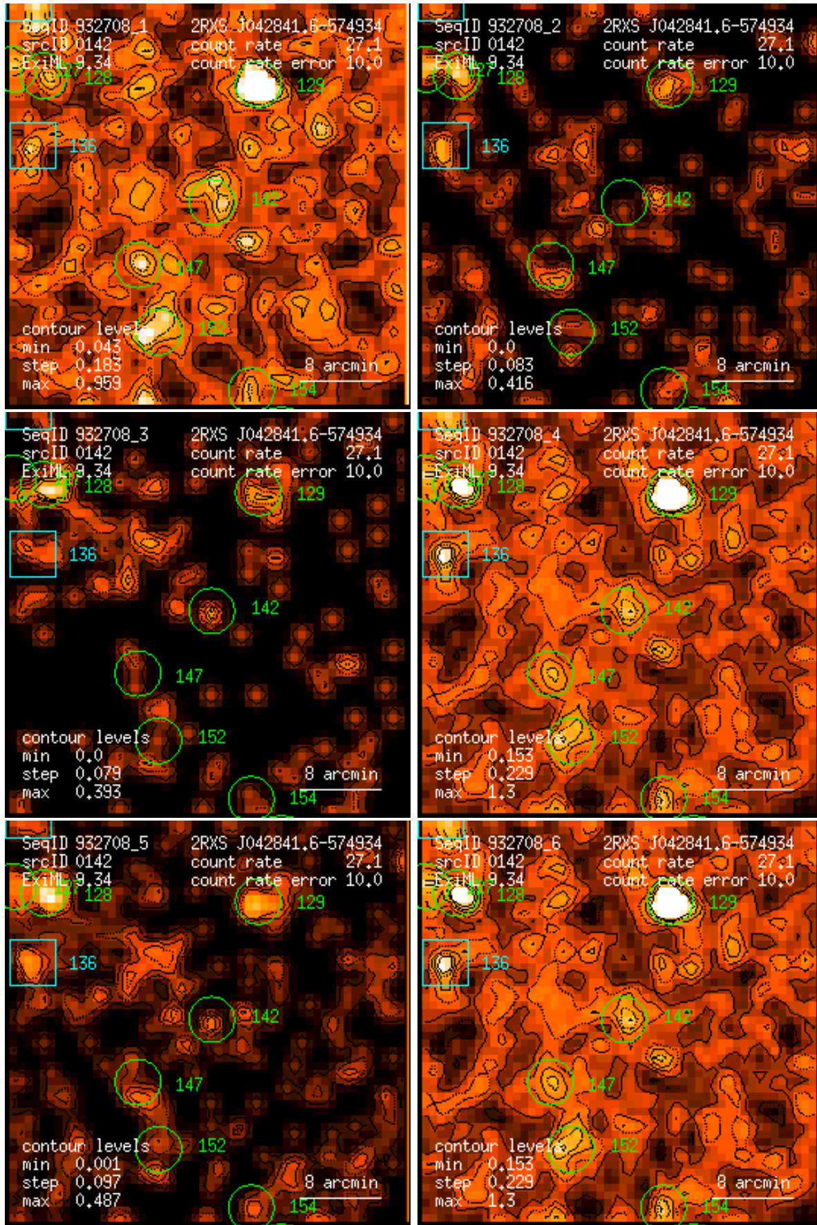
Figure 142: RASS 932708: detection 0142: band rate images, Gaussian filter: (1) PSPC channels 11 – 41, (2) 52 – 90, (3) 91 – 201, (4) 11 – 235, (5) 52 – 201, (6) 11 – 201. Broad band rates in counts/ks. Band rate contour levels in counts/ks/arcmin 2 .
