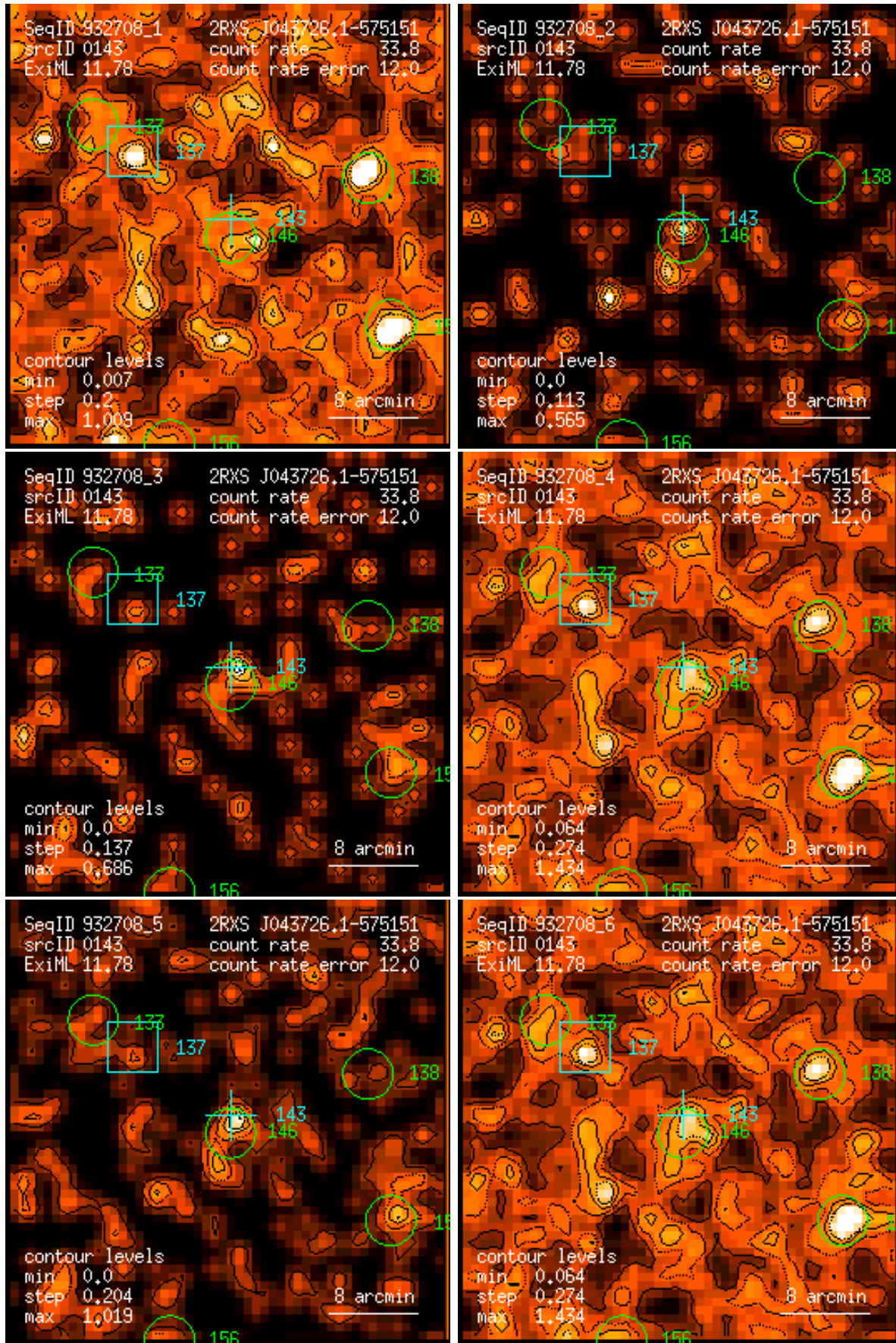
Figure 143: RASS 932708: detection 0143: band rate images, Gaussian filter: (1) PSPC channels 11 – 41, (2) 52 – 90, (3) 91 – 201, (4) 11 – 235, (5) 52 – 201, (6) 11 – 201. Broad band rates in counts/ks. Band rate contour levels in counts/ks/arcmin 2 .
