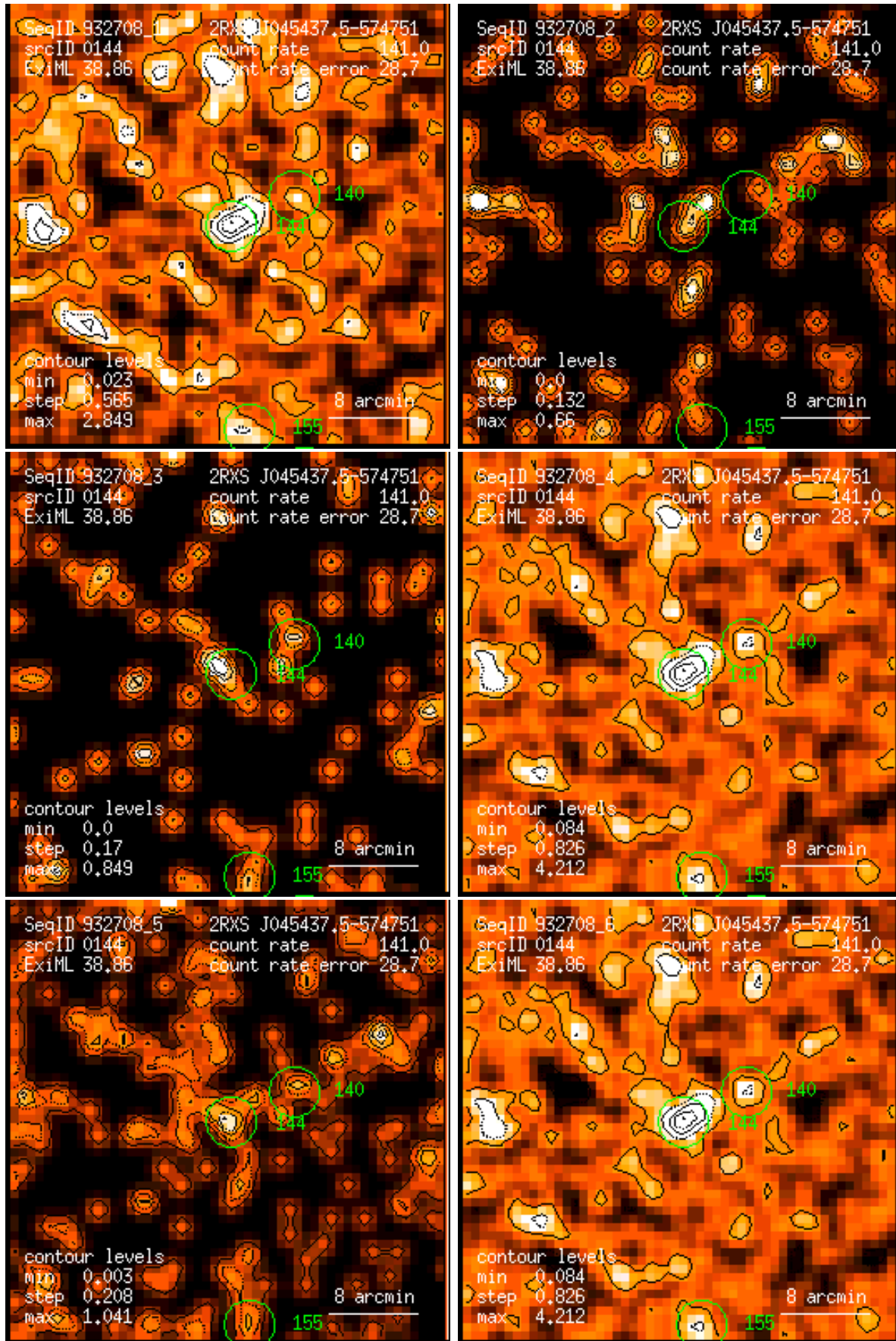
Figure 144: RASS 932708: detection 0144: band rate images, Gaussian filter: (1) PSPC channels 11 – 41, (2) 52 – 90, (3) 91 – 201, (4) 11 – 235, (5) 52 – 201, (6) 11 – 201. Broad band rates in counts/ks. Band rate contour levels in counts/ks/arcmin 2 .
