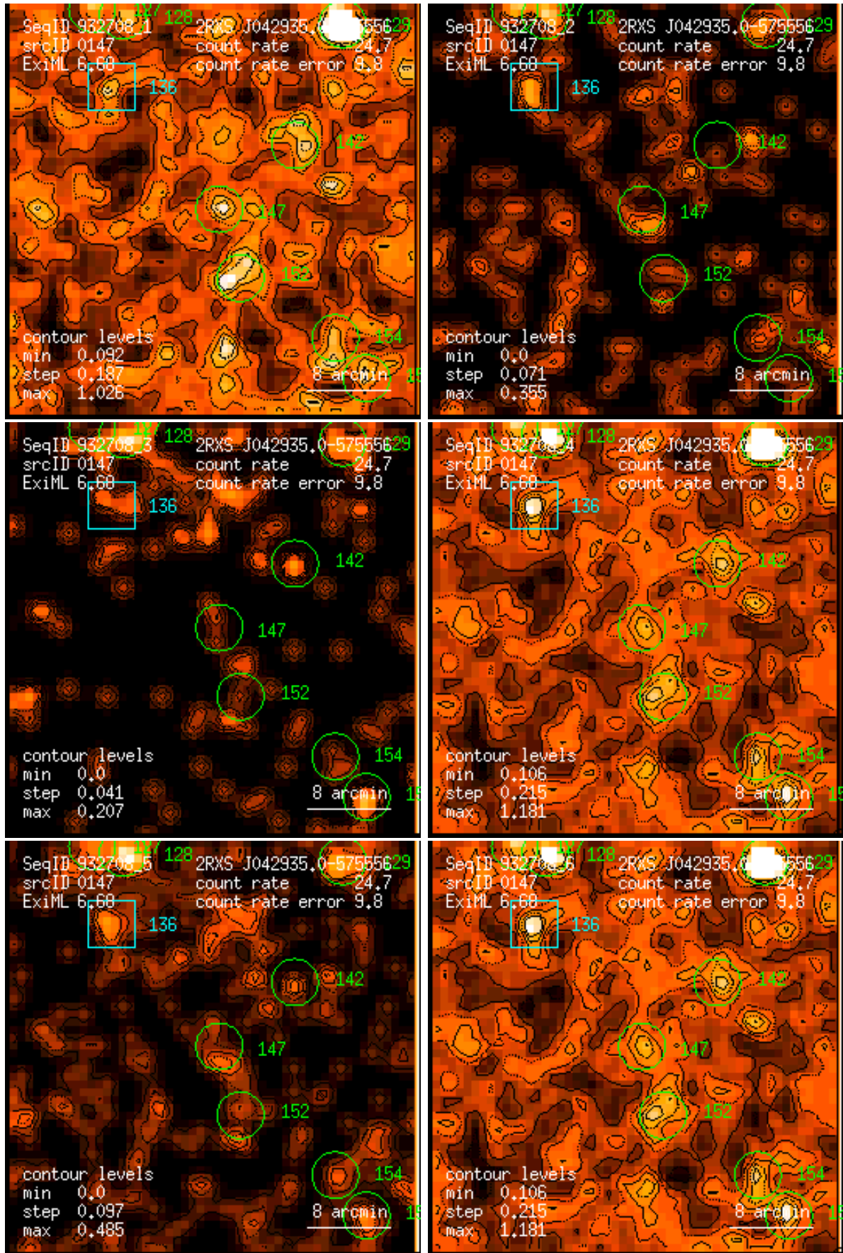
Figure 147: RASS 932708: detection 0147: band rate images, Gaussian filter: (1) PSPC channels 11 – 41, (2) 52 – 90, (3) 91 – 201, (4) 11 – 235, (5) 52 – 201, (6) 11 – 201. Broad band rates in counts/ks. Band rate contour levels in counts/ks/arcmin 2 .
