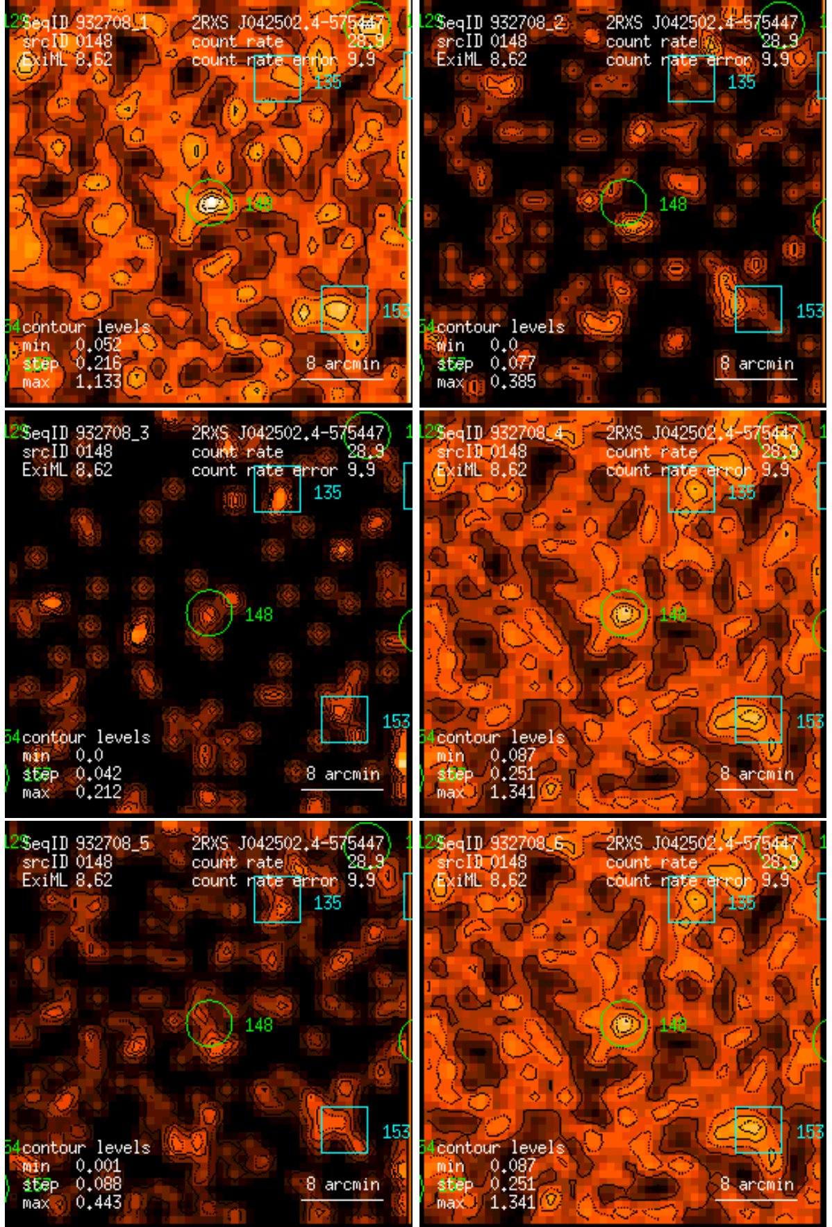
Figure 148: RASS 932708: detection 0148: band rate images, Gaussian filter: (1) PSPC channels 11 – 41, (2) 52 – 90, (3) 91 – 201, (4) 11 – 235, (5) 52 – 201, (6) 11 – 201. Broad band rates in counts/ks. Band rate contour levels in counts/ks/arcmin 2 .
