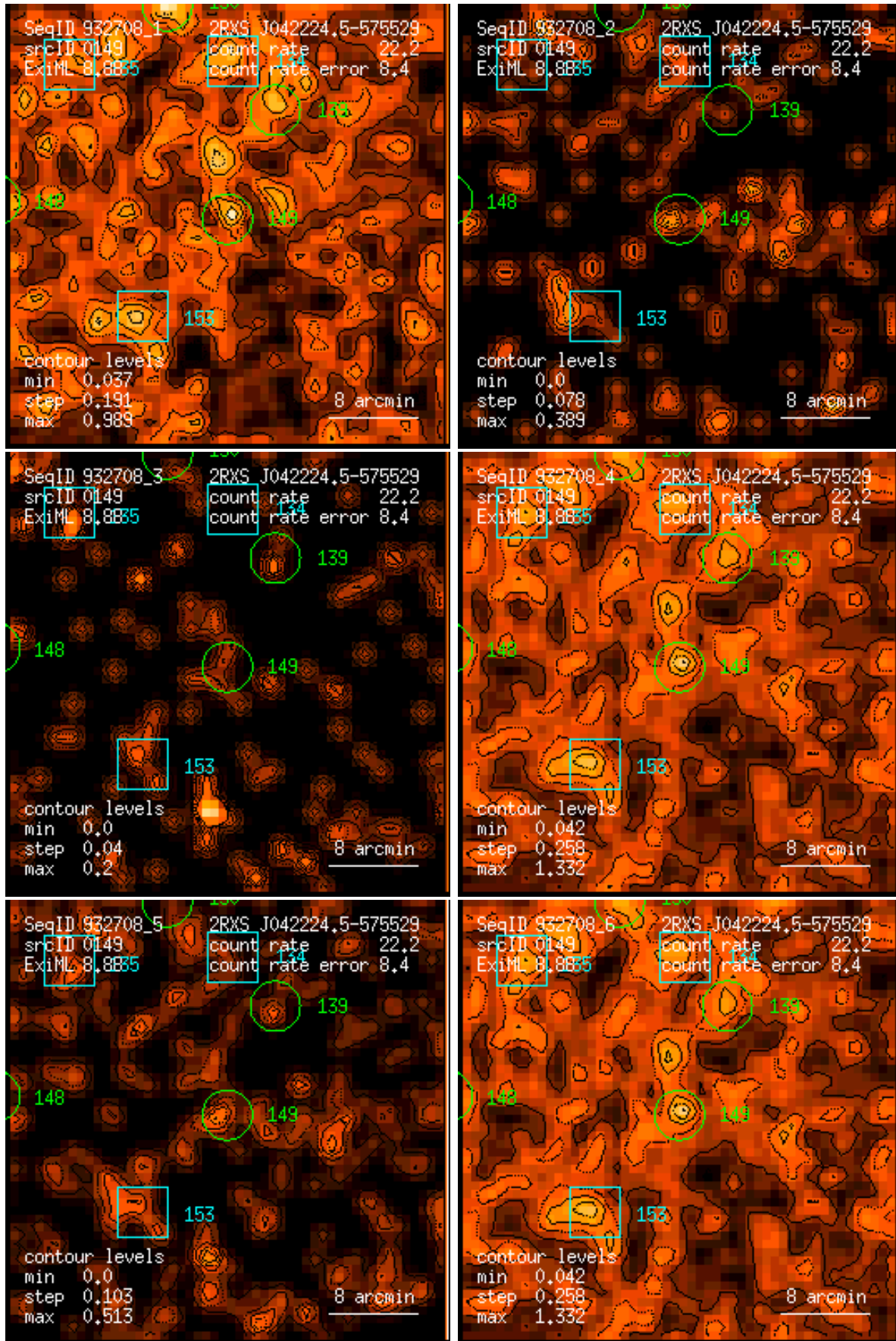
Figure 149: RASS 932708: detection 0149: band rate images, Gaussian filter: (1) PSPC channels 11 – 41, (2) 52 – 90, (3) 91 – 201, (4) 11 – 235, (5) 52 – 201, (6) 11 – 201. Broad band rates in counts/ks. Band rate contour levels in counts/ks/arcmin 2 .
