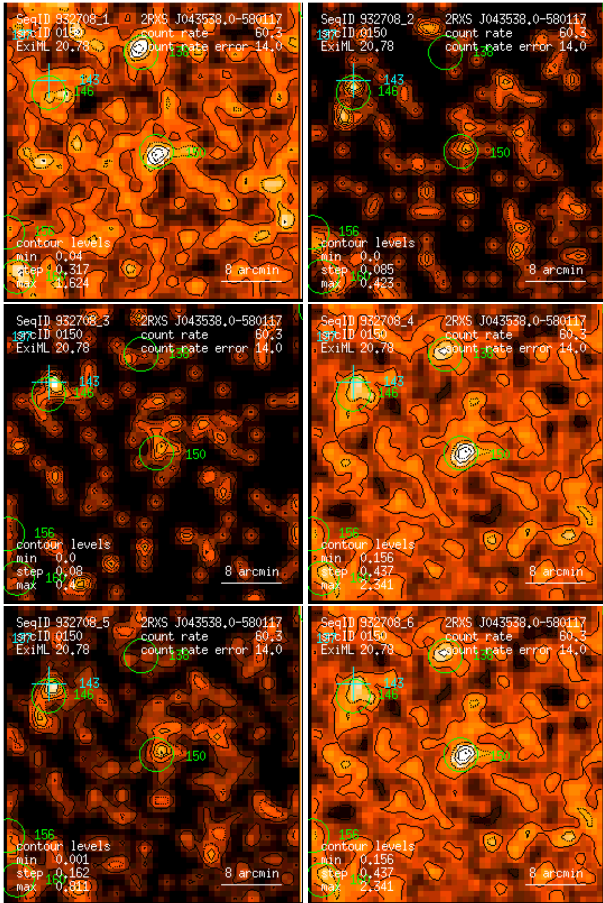
Figure 150: RASS 932708: detection 0150: band rate images, Gaussian filter: (1) PSPC channels 11 – 41, (2) 52 – 90, (3) 91 – 201, (4) 11 – 235, (5) 52 – 201, (6) 11 – 201. Broad band rates in counts/ks. Band rate contour levels in counts/ks/arcmin 2 .
