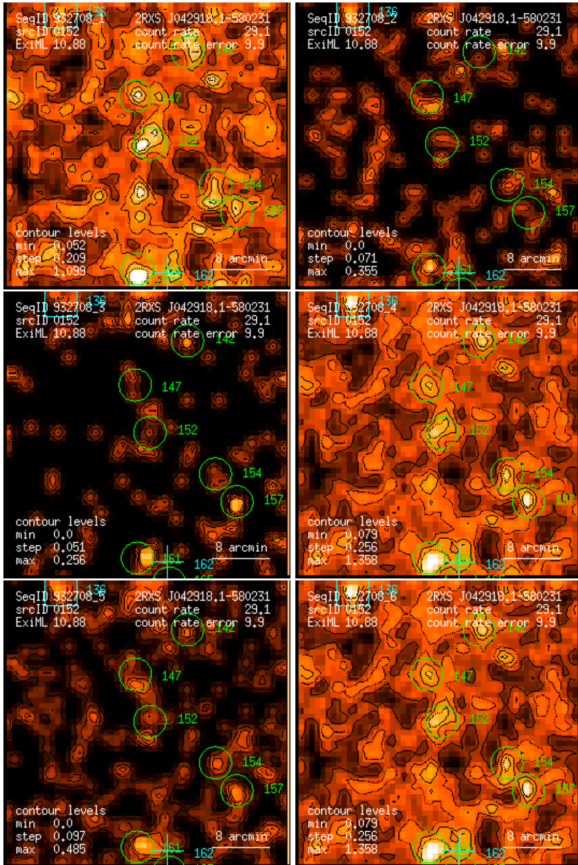
Figure 152: RASS 932708: detection 0152: band rate images, Gaussian filter: (1) PSPC channels 11 – 41, (2) 52 – 90, (3) 91 – 201, (4) 11 – 235, (5) 52 – 201, (6) 11 – 201. Broad band rates in counts/ks. Band rate contour levels in counts/ks/arcmin 2 .
