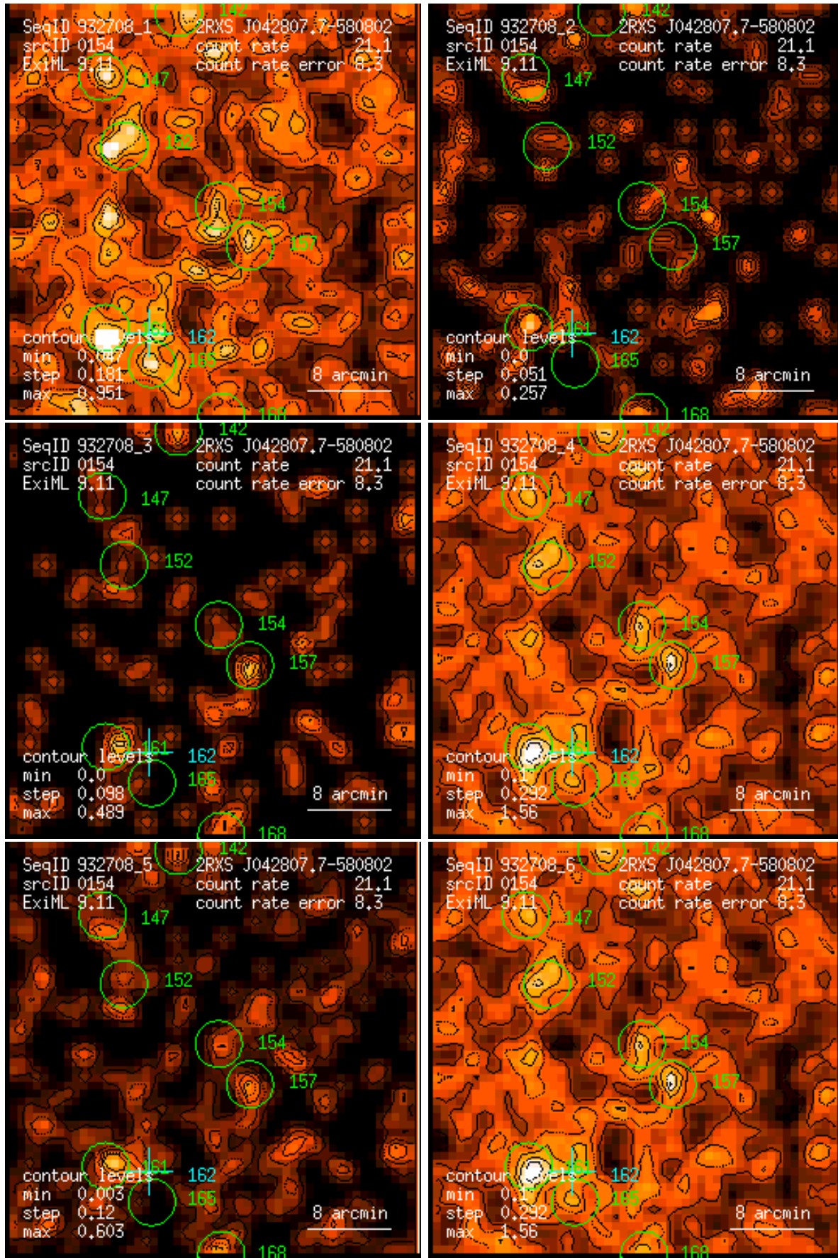
Figure 154: RASS 932708: detection 0154: band rate images, Gaussian filter: (1) PSPC channels 11 – 41, (2) 52 – 90, (3) 91 – 201, (4) 11 – 235, (5) 52 – 201, (6) 11 – 201. Broad band rates in counts/ks. Band rate contour levels in counts/ks/arcmin 2 .
